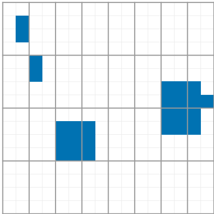
a VSA selects on 64-token tiles — 10% kept
