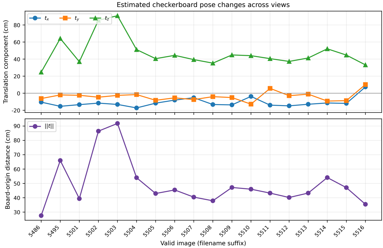
Figure 4: Translation-vector variation across views. OpenCV uses \mathbf{t} to map the checkerboard origin from board coordinates to camera coordinates; because the object-point square size is 3 cm, the plotted components and \|\mathbf{t}\| are in centimeters. The t_z curve is the depth of the board origin, while the lower panel gives its Euclidean distance from the camera origin.
