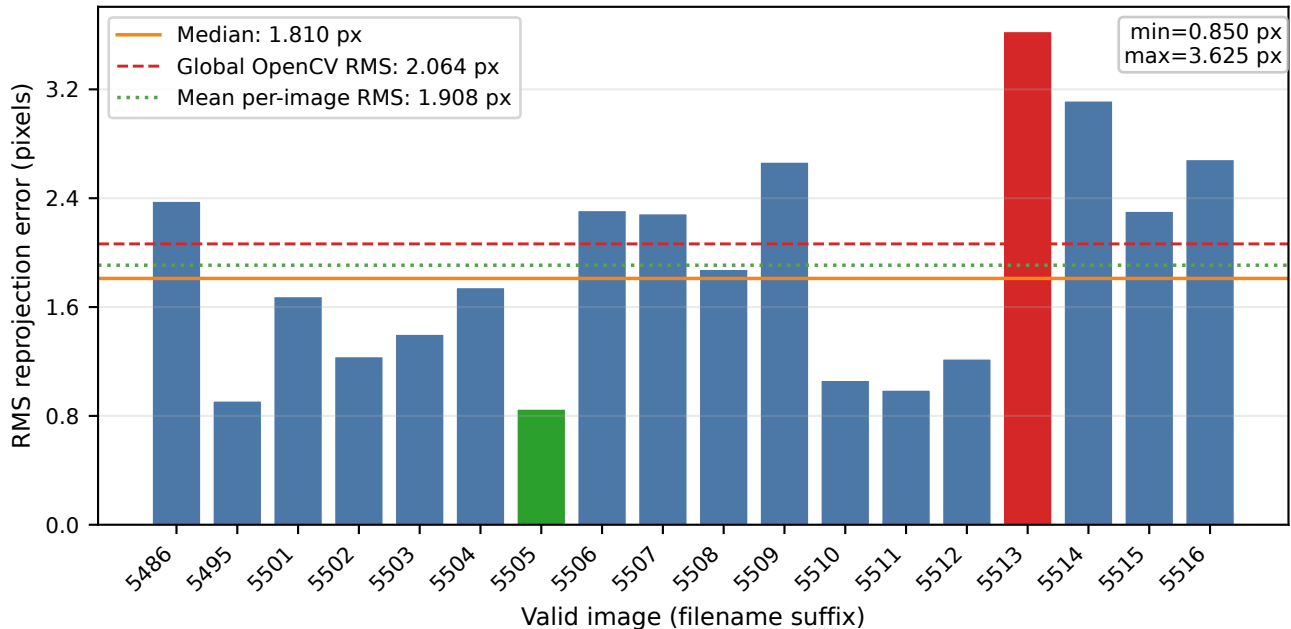
Reprojection error varies across the 18 valid views
