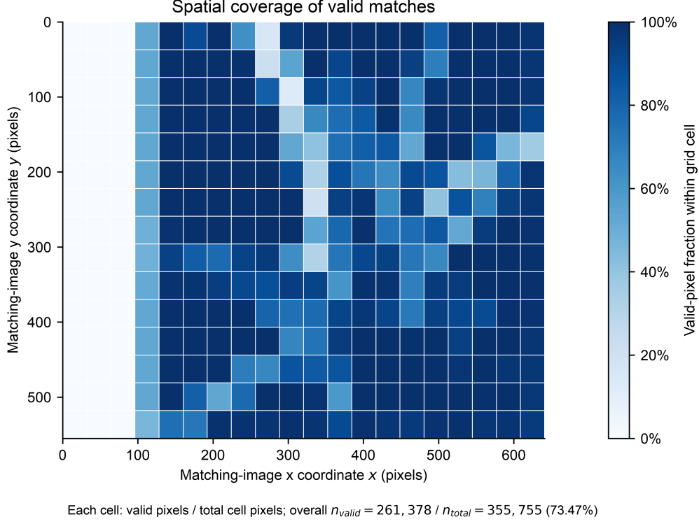
Figure 4: Spatial valid-matching coverage. Color denotes the proportion of pixels with finite disparity and d > 15 px in each cell of the 15 \times 20 grid. The calculation covers all 261378 valid pixels, giving an overall coverage of 73.4713%.
