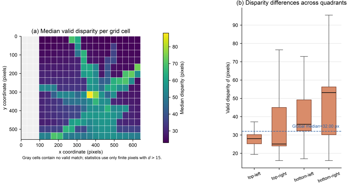
Figure 6: Spatial disparity and quadrant comparison. (a) Color denotes the median valid disparity within each grid cell; gray denotes no valid match. (b) Box plots of all valid disparities in the four quadrants; the box spans P_{25} – P_{75} and the horizontal line marks the median. The quadrants are defined only by image coordinates and do not represent semantic object classes.
