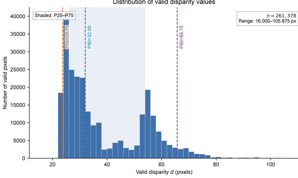
Figure 5: Distribution of valid disparities ( n = 261378 ). Statistics use only finite pixels with d > 15 px; the shaded region denotes P_{25} – P_{75} , and dashed lines mark P_{05} , the median, and P_{95} . The horizontal axis is measured in pixels.
