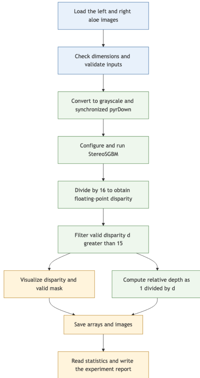
Figure 1: Stereo depth estimation pipeline generated from the Mermaid source file.
