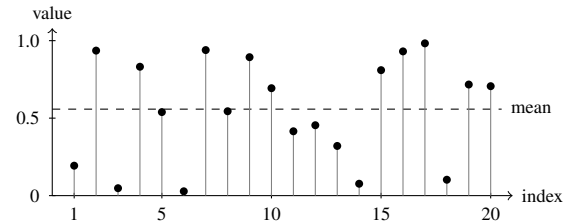
Fig. 5. The 20 printed RandomVector values in output order; the dashed line is the reported mean, 0.55804.
