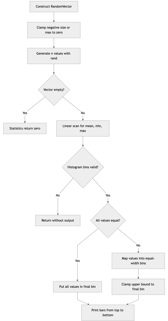
Fig. 2. RandomVector generation, statistics, and histogram output.
