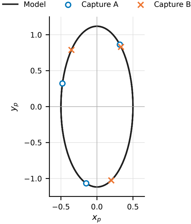
Fig. 6. Analytic relative ellipse and six TF samples in the plane coordinates of Eq. (13). Symbols distinguish the two captures in Table II.
