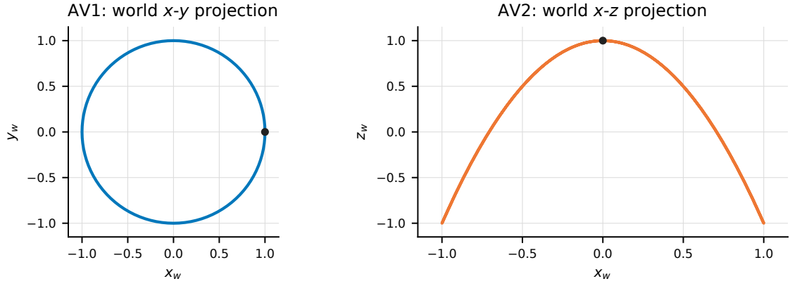
Fig. 3. Analytic world-frame projections over 0 \leq t \leq 2\pi . Black markers show the starting positions at t = 0 ; the curves are calculated from Eq. (1), not extracted from RViz.
