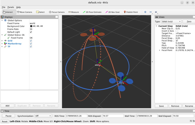
Fig. 2. Dynamic trajectories visualized in RViz with the fixed frame set to world.
