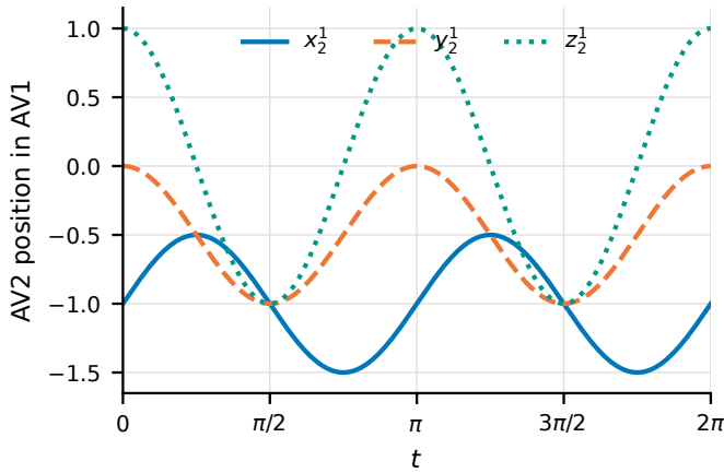
Fig. 5. Analytic components of AV2's position in AV1 from Eq. (8). The interval 0 \leq t \leq 2\pi contains two relative-motion cycles.
