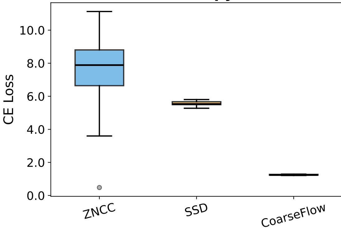
Cross-Entropy Loss
