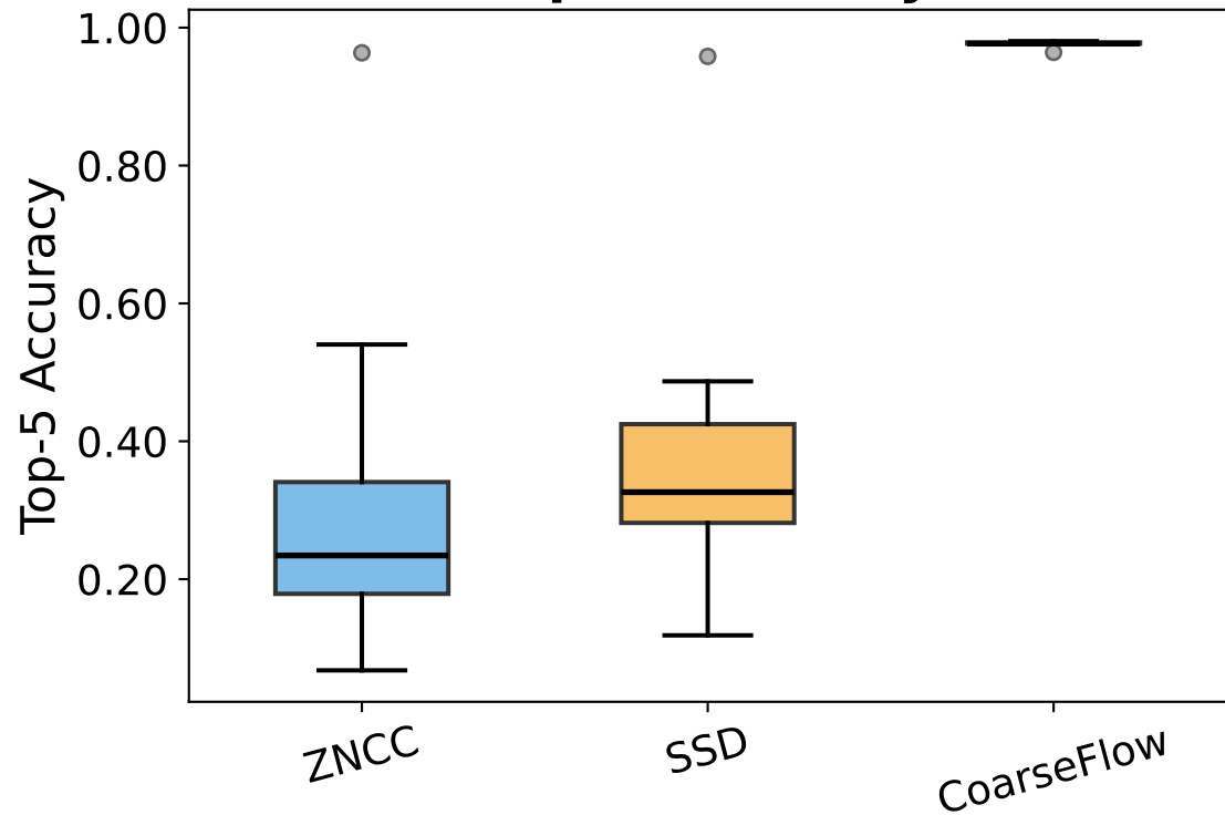
Top-5 Accuracy
