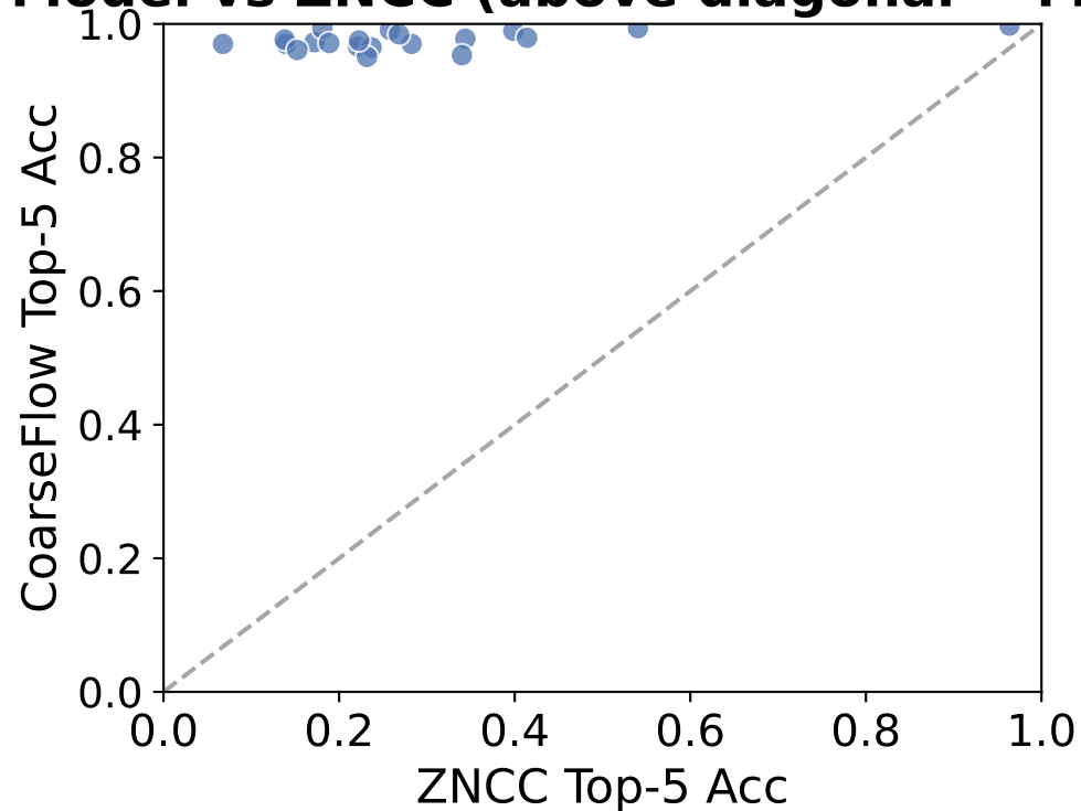
Top-5: Model vs ZNCC (above diagonal = Model wins)
