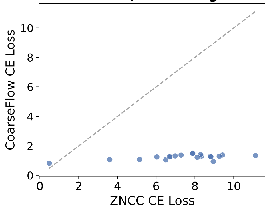
CE Loss: Model vs ZNCC (below diagonal = Model wins)
