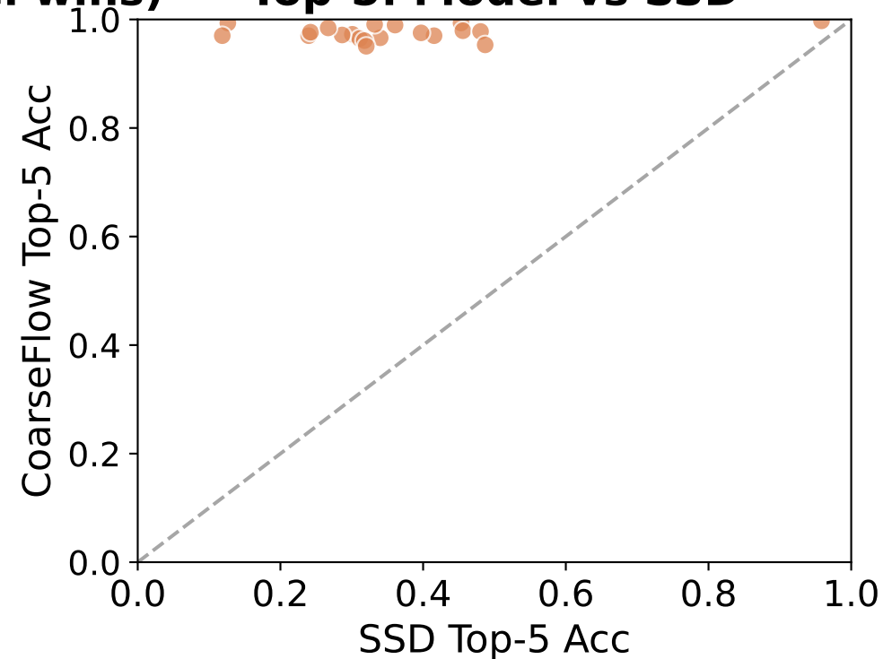
Top-5: Model vs SSD
