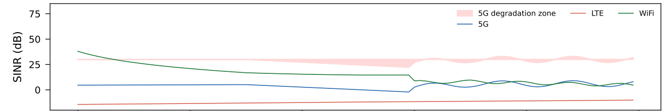
LAAVHA (fixed \Delta_{th}=0.05 ): 24 HO
