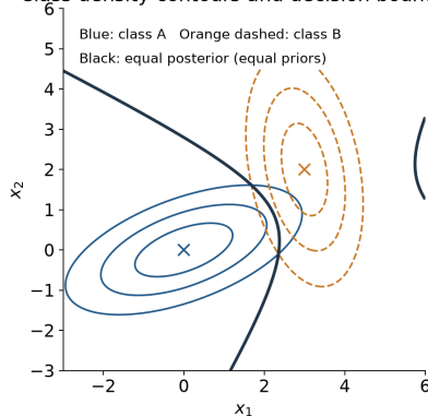
Class density contours and decision boundary
