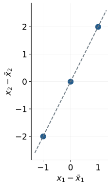
Centred observations confined to one direction
