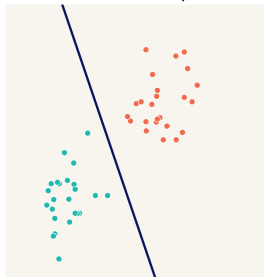
Before the extreme point
