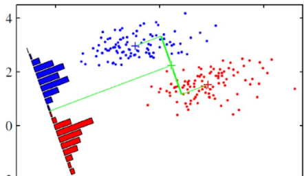
Projection onto z = w^T x
