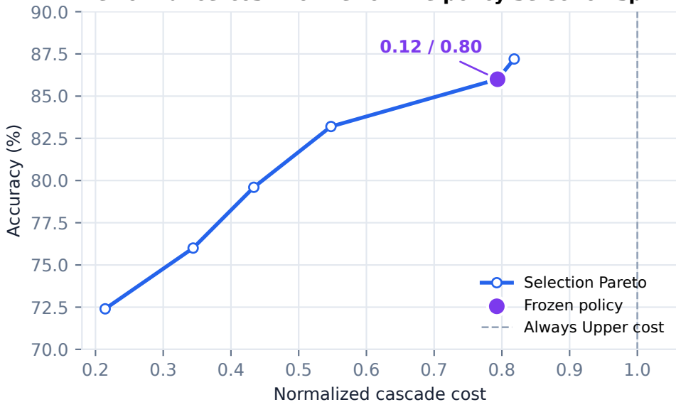
Performance-cost frontier on the policy-selection split
