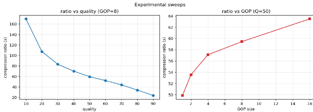
Figure 2 — Compression ratio as a function of the Quantisation Factor (left) and of the GOP size (right).
