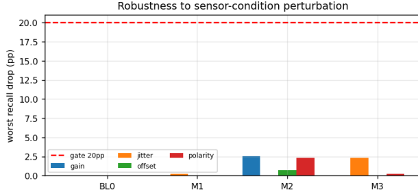
Figure 2: Robustness to benign measurement perturbation. Models that are indistinguishable in Table 3 differ by more than 5\times .
