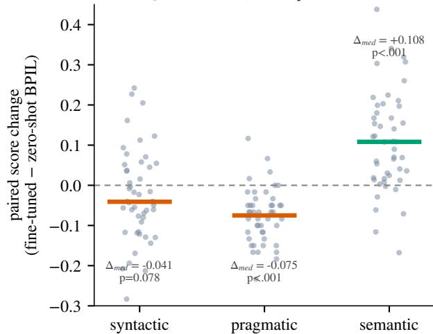
Qwen2.5-14B (n = 48 paired items)
