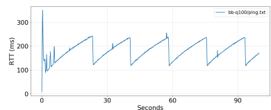
RTT (q=100)
