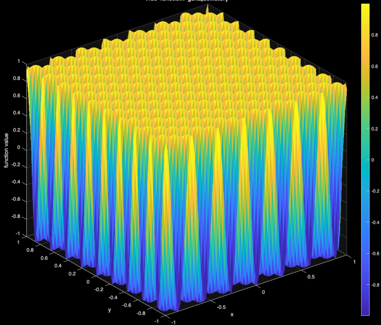
True function: genz_oscillatory
