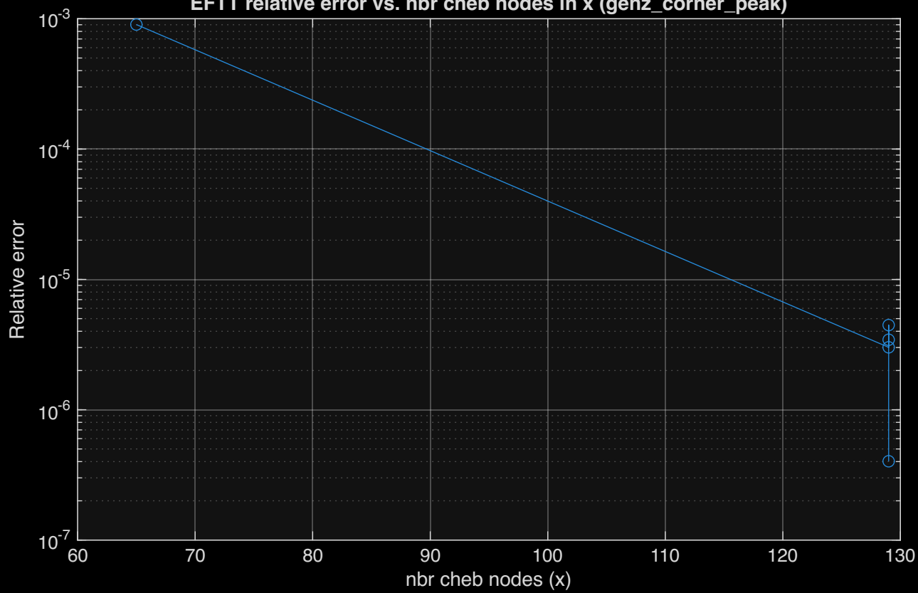
EFTT relative error vs. nbr cheb nodes in x (genz_corner_peak)
