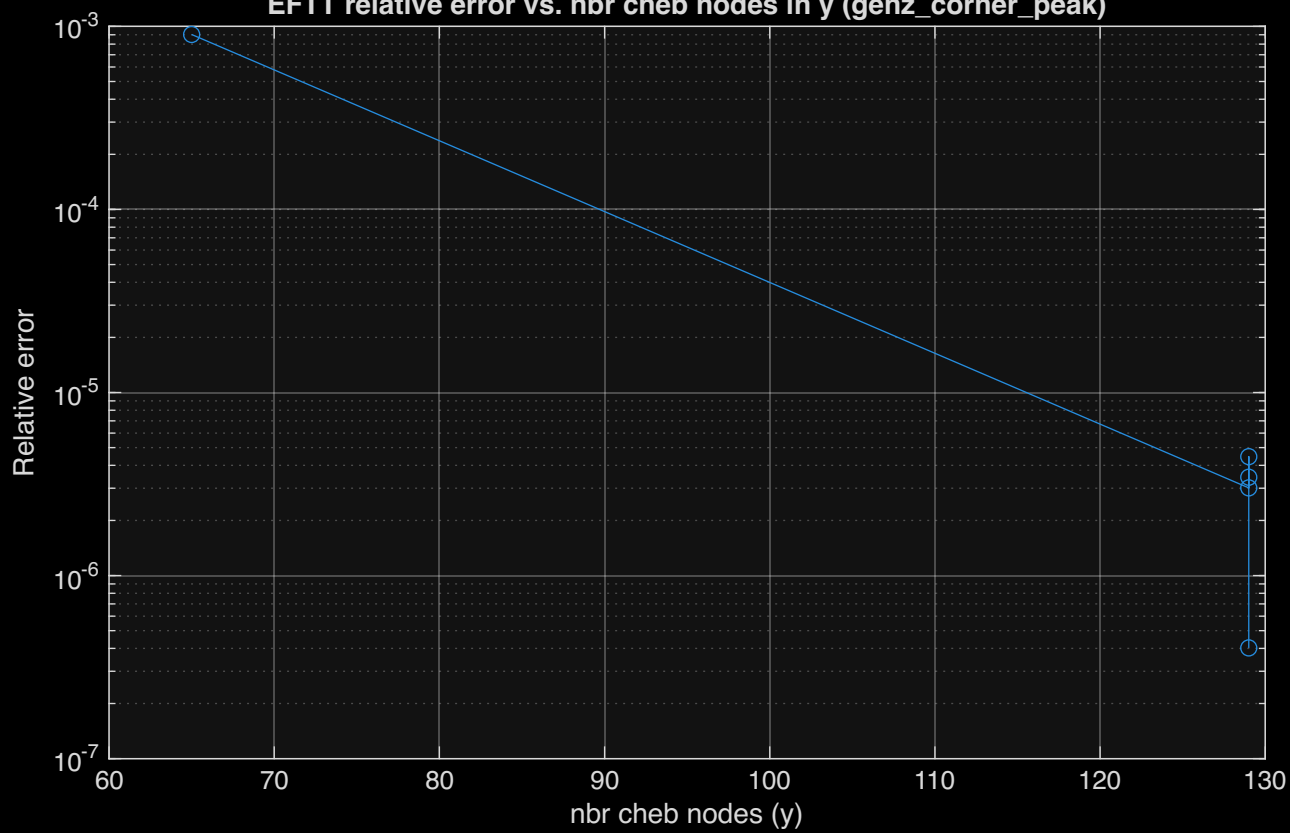
EFTT relative error vs. nbr cheb nodes in y (genz_corner_peak)
