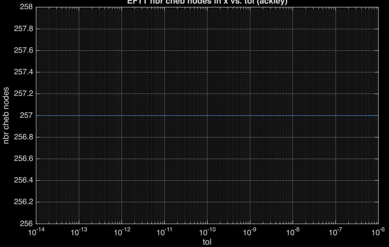
EFTT nbr cheb nodes in x vs. tol (ackley)
