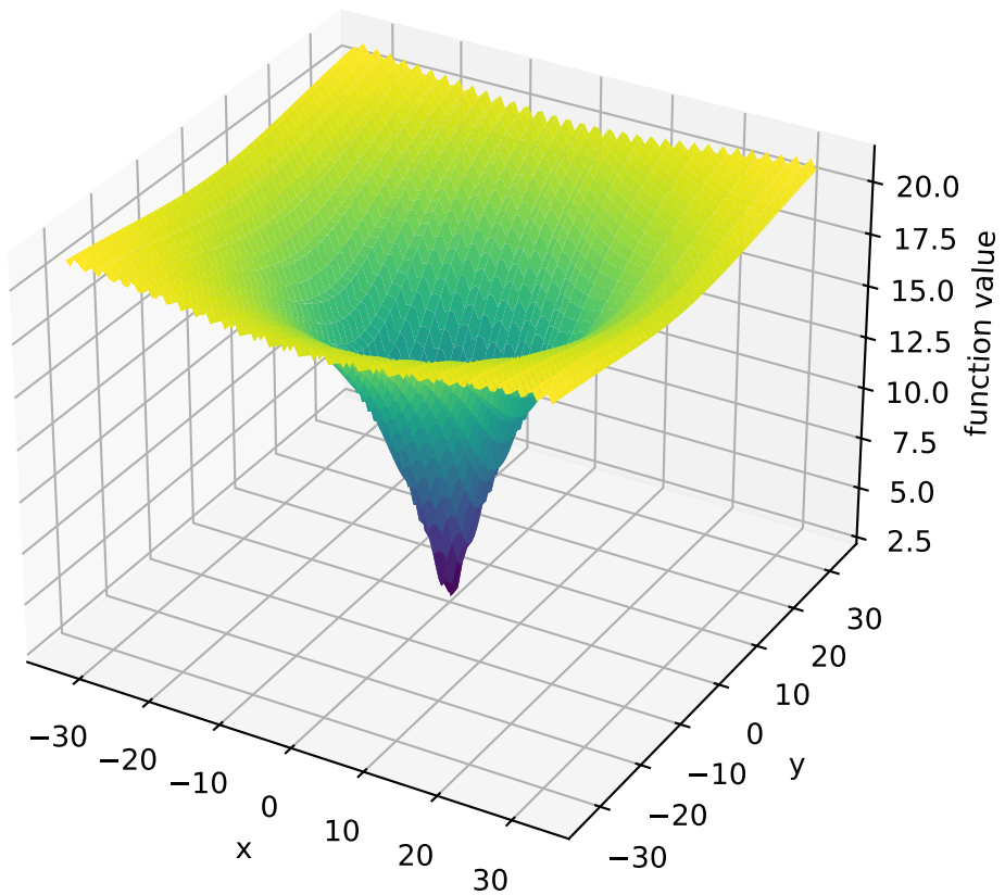
True function: ackley
