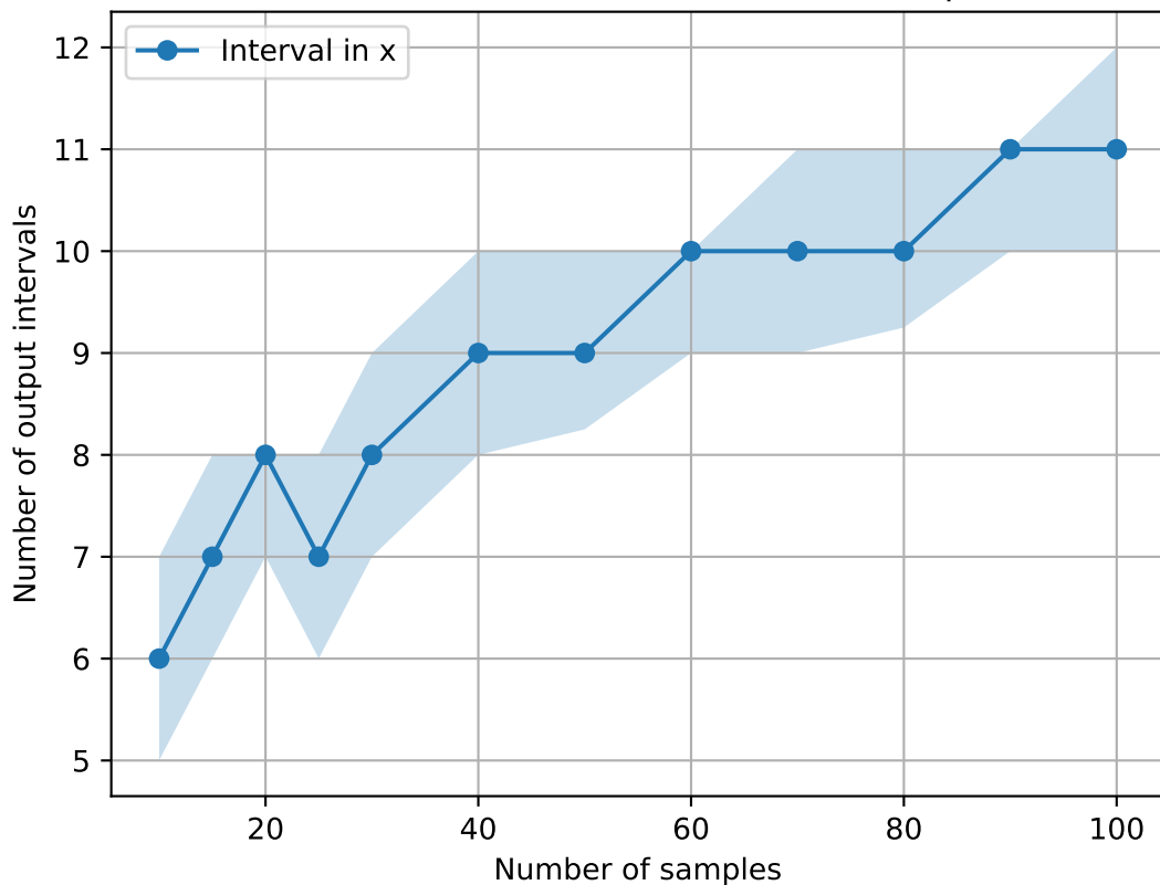
Number of intervals versus number of samples in x
