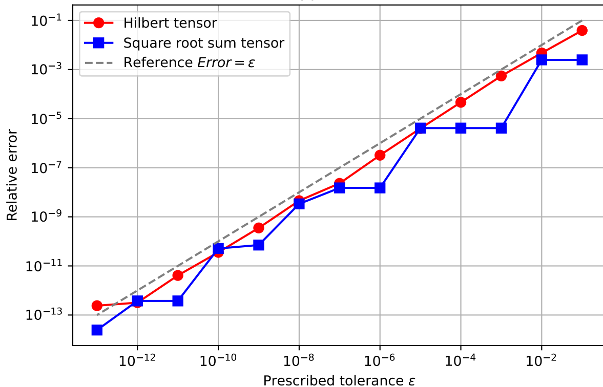
TT-SVD approximation error
