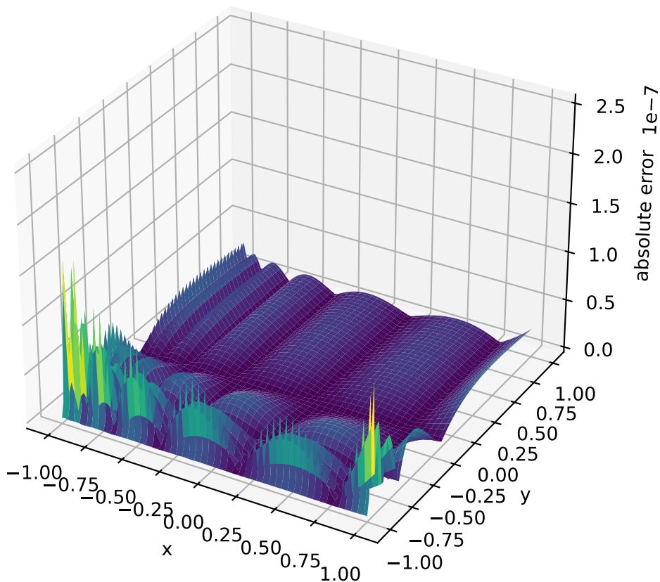
Absolute error: genz_corner_peak
