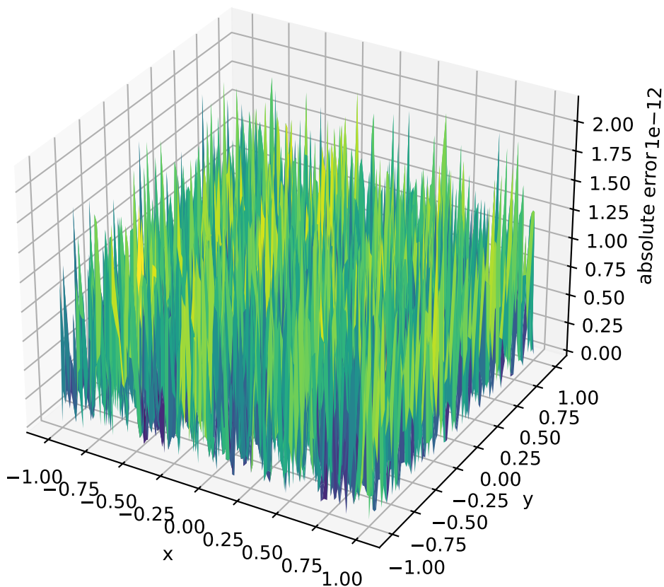
Absolute error: genz_oscillatory
