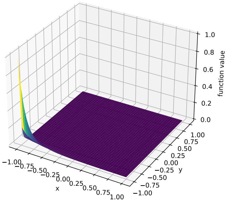
True function: genz_corner_peak
