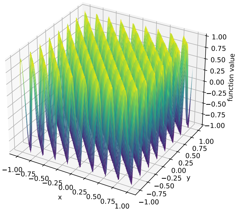
True function: genz_oscillatory
