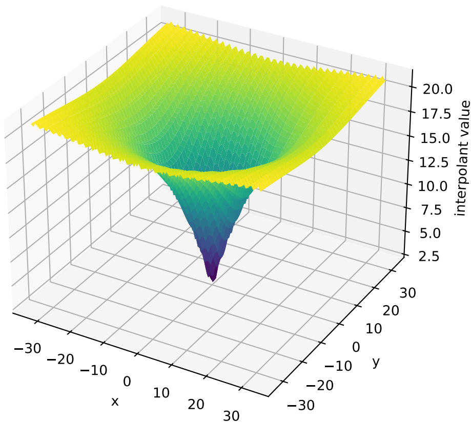
Interpolant: ackley
