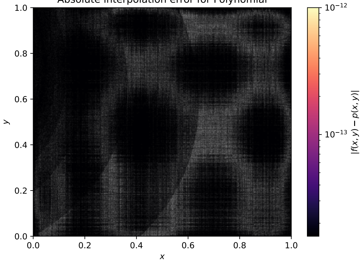
Absolute interpolation error for Polynomial
