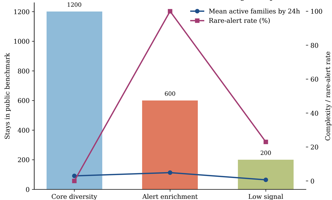
Soft-balanced 2k benchmark mixes dense and low-signal trajectories
