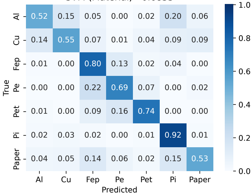
SVM (Material) - 0.6833
