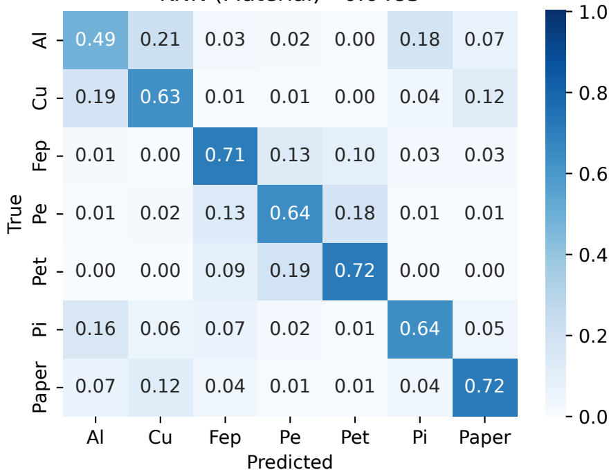
KNN (Material) - 0.6483
