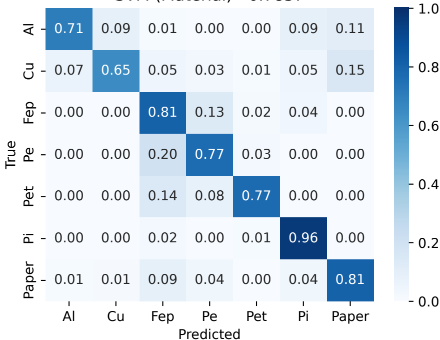
SVM (Material) - 0.7837
