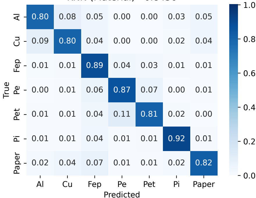
KNN (Material) - 0.8456
