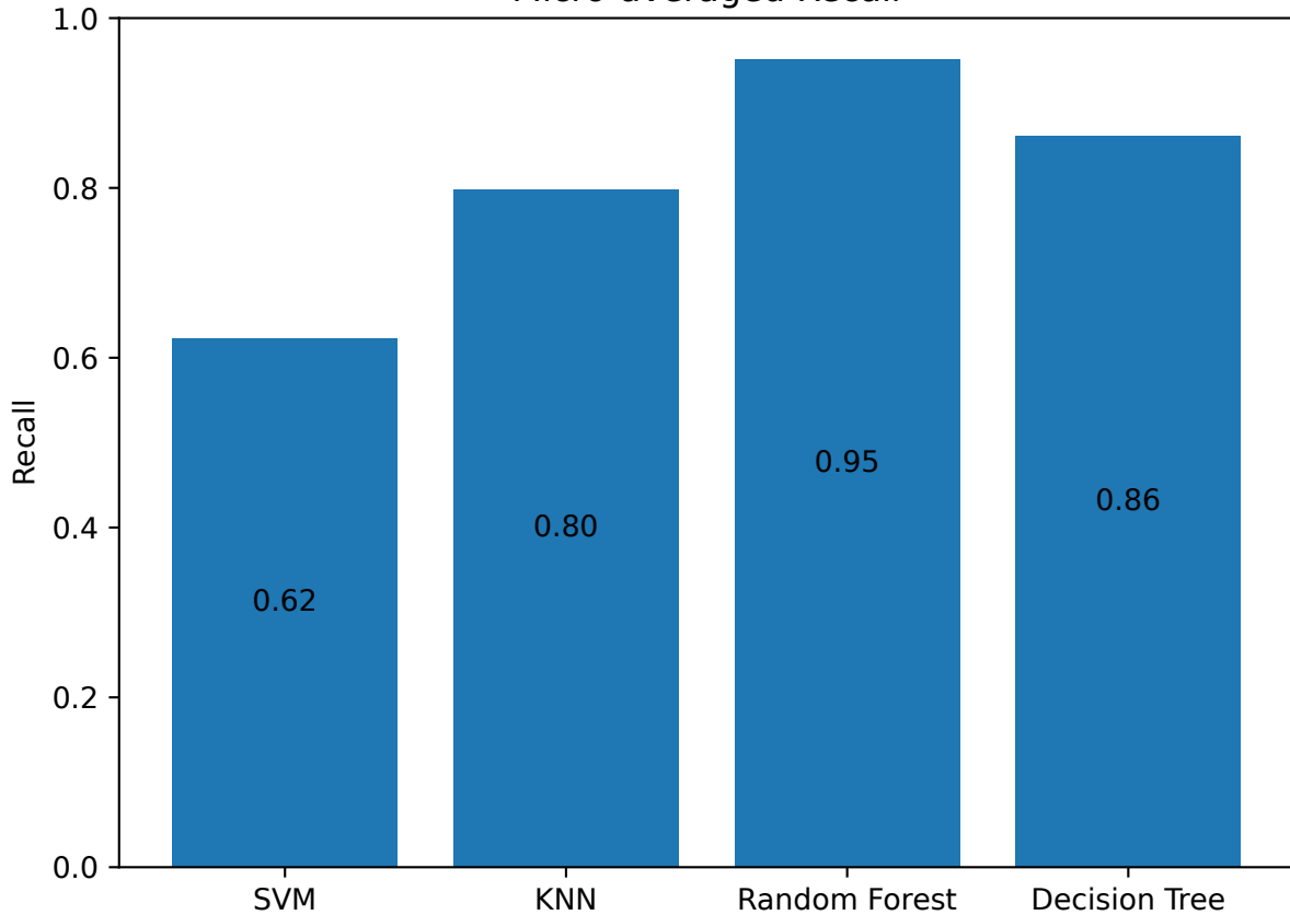
Micro-averaged Recall
