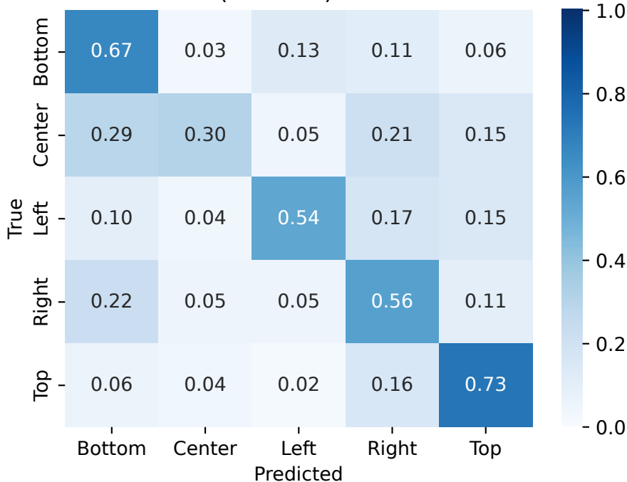
SVM (Location) - 0.5631
