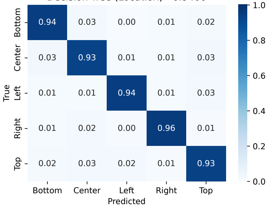
Decision Tree (Location) - 0.9400
