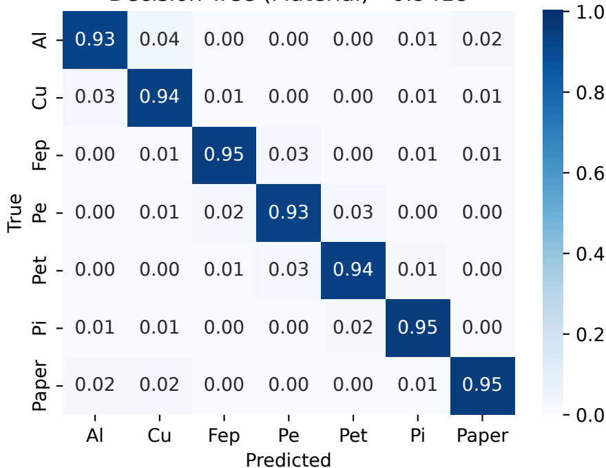
Decision Tree (Material) - 0.9418
