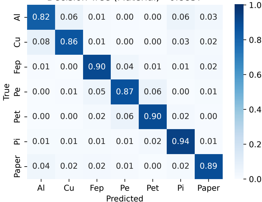
Decision Tree (Material) - 0.8837
