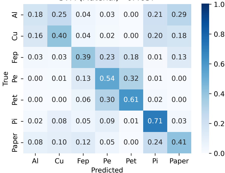
SVM (Material) - 0.4637
