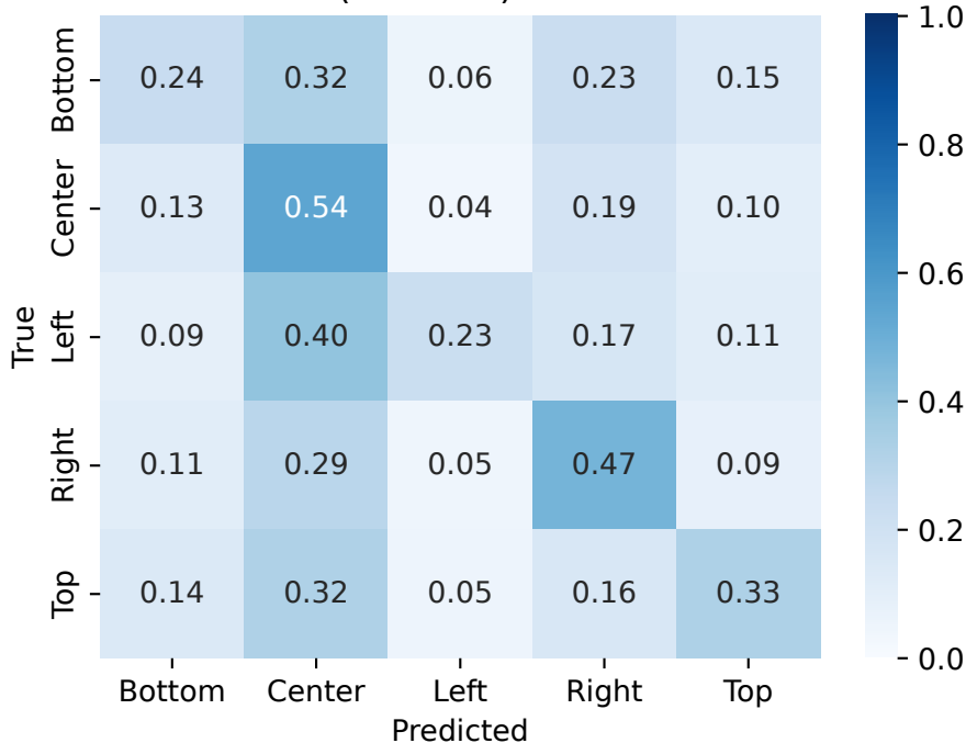
SVM (Location) - 0.3601
