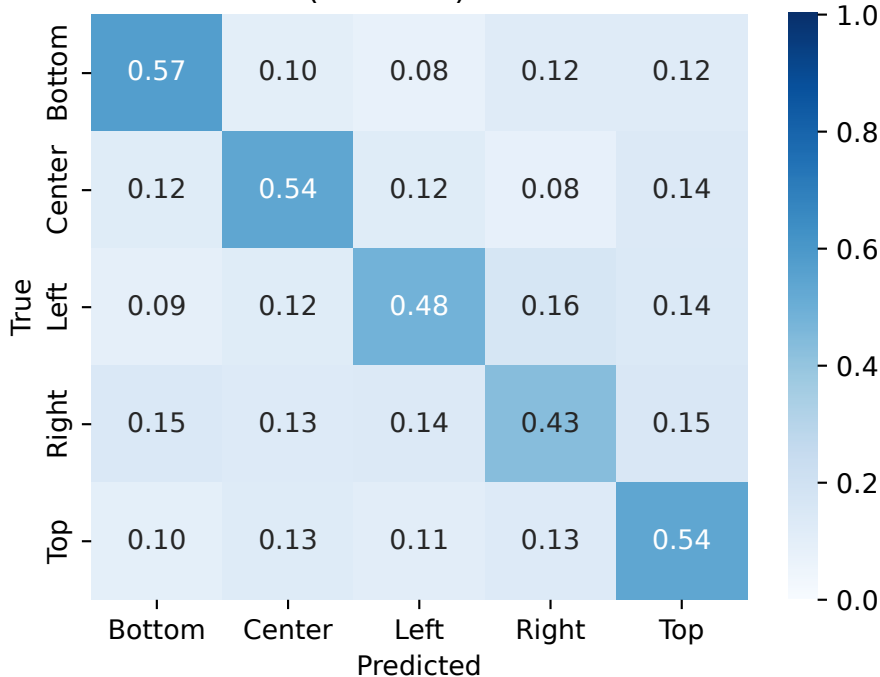
KNN (Location) - 0.5122
