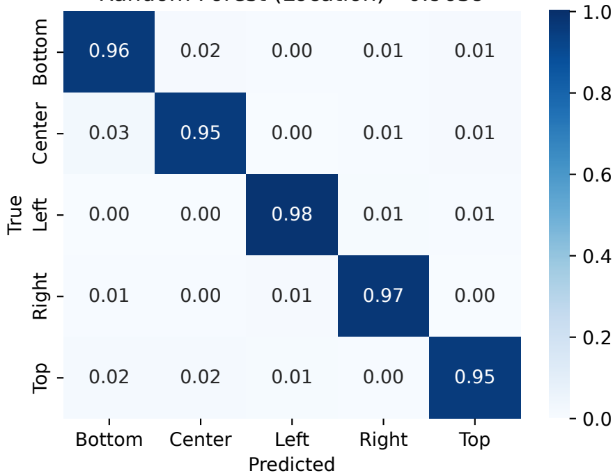
Random Forest (Location) - 0.9639
