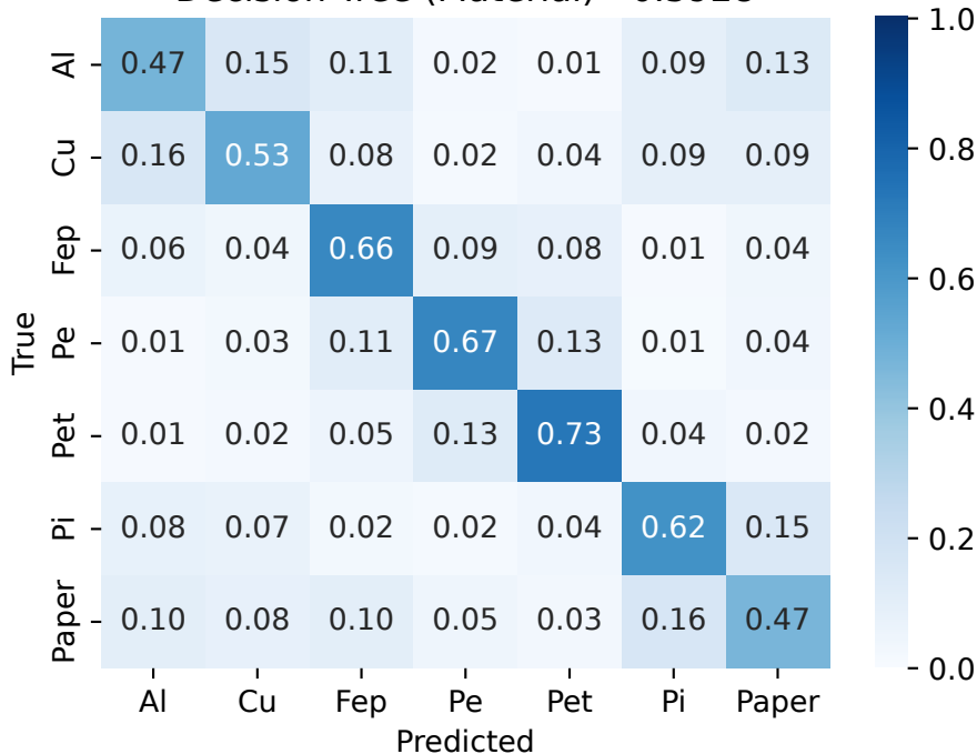
Decision Tree (Material) - 0.5928
