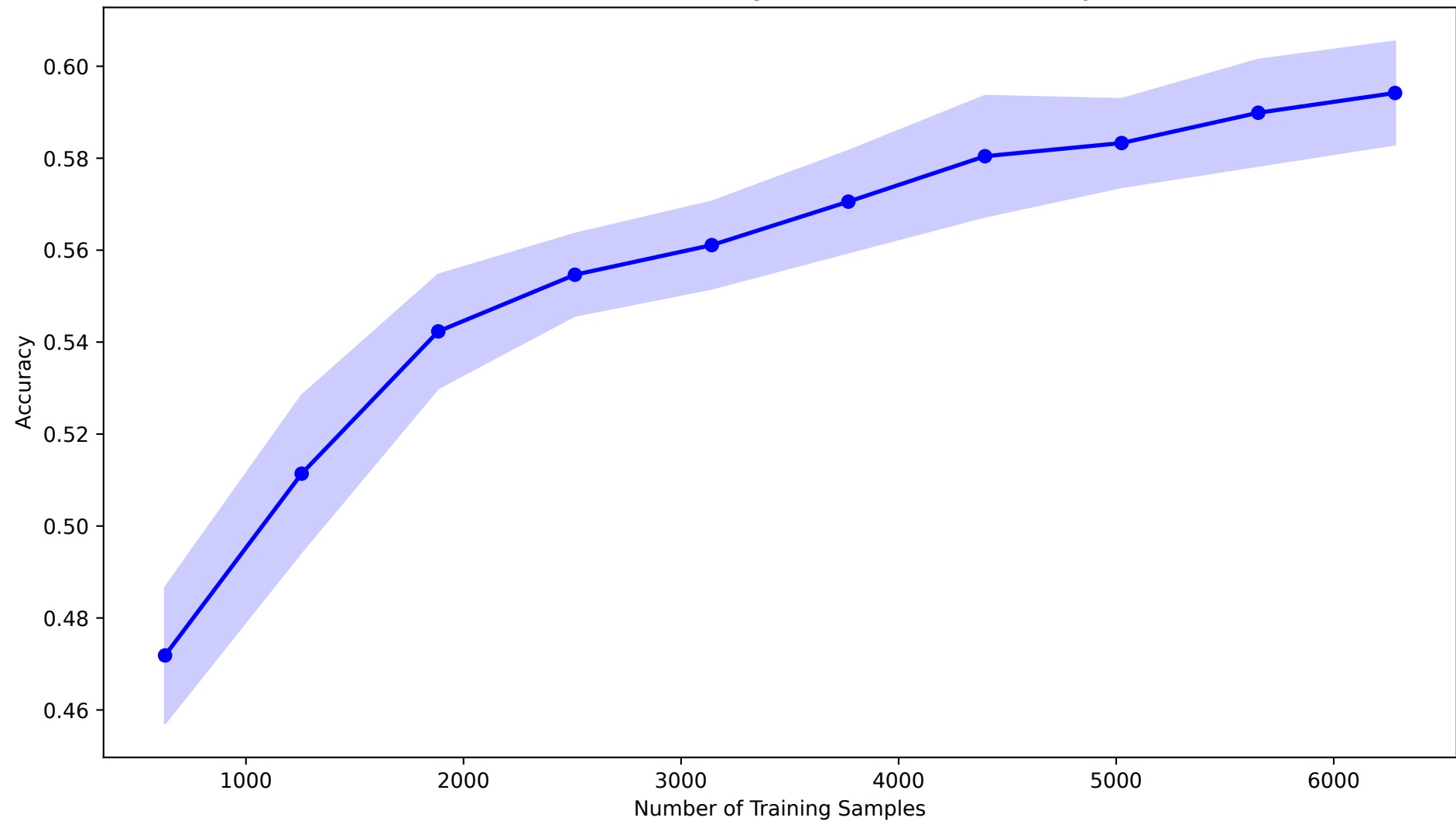
Random Forest Learning Curve - Location Accuracy
