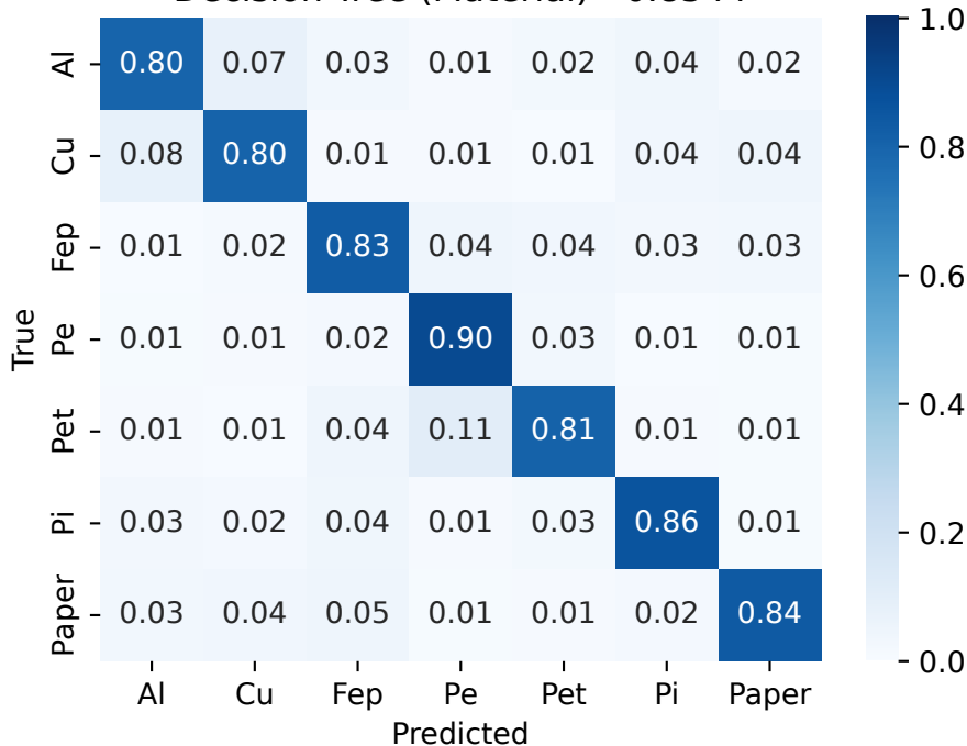
Decision Tree (Material) - 0.8344
