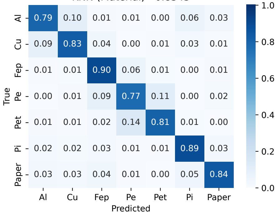
KNN (Material) - 0.8343
