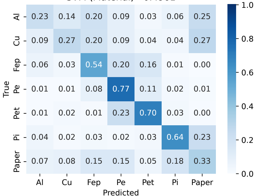
SVM (Material) - 0.4961
