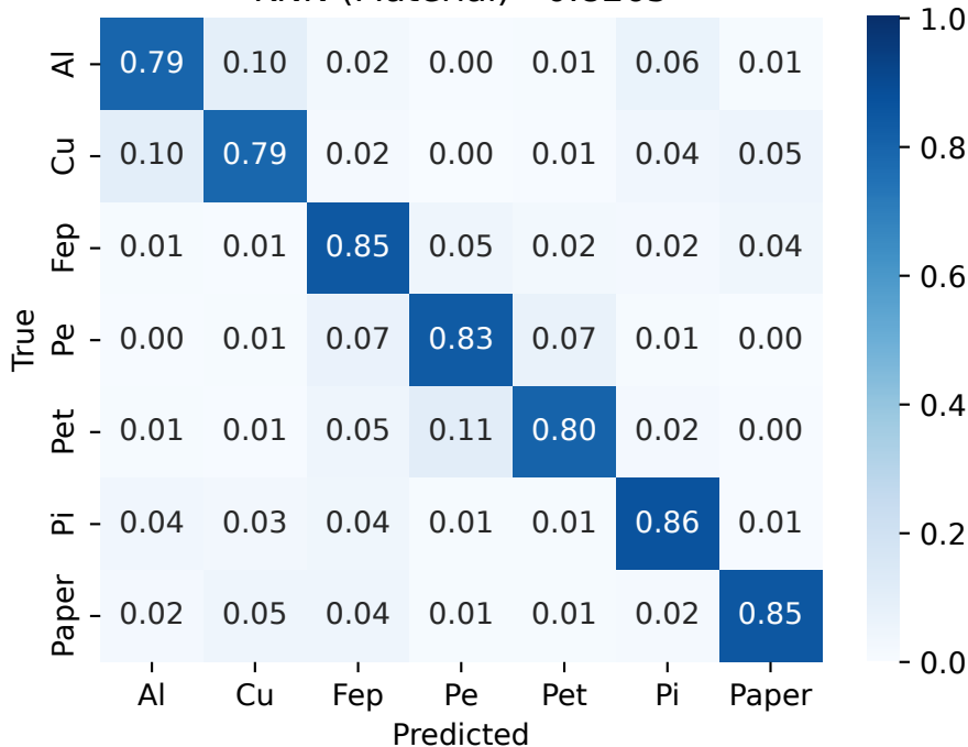
KNN (Material) - 0.8265
