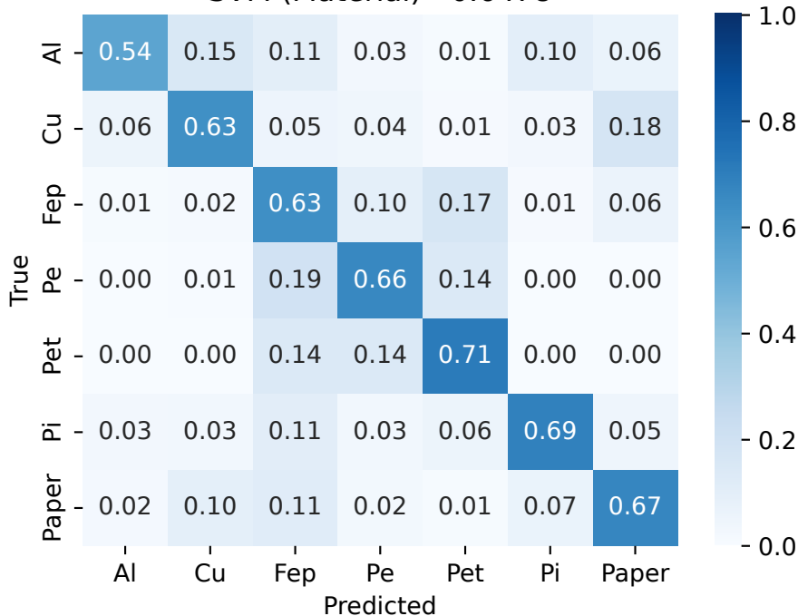
SVM (Material) - 0.6478
