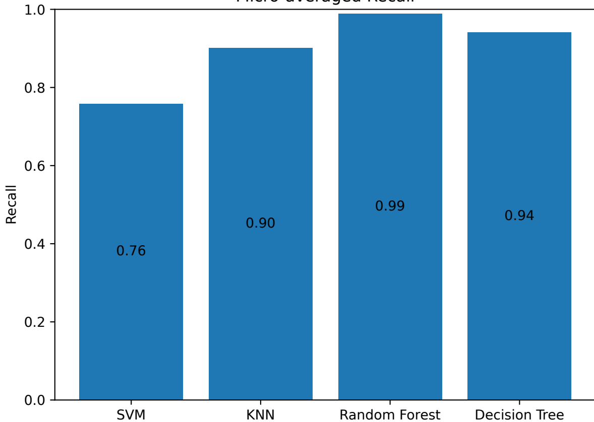
Micro-averaged Recall
