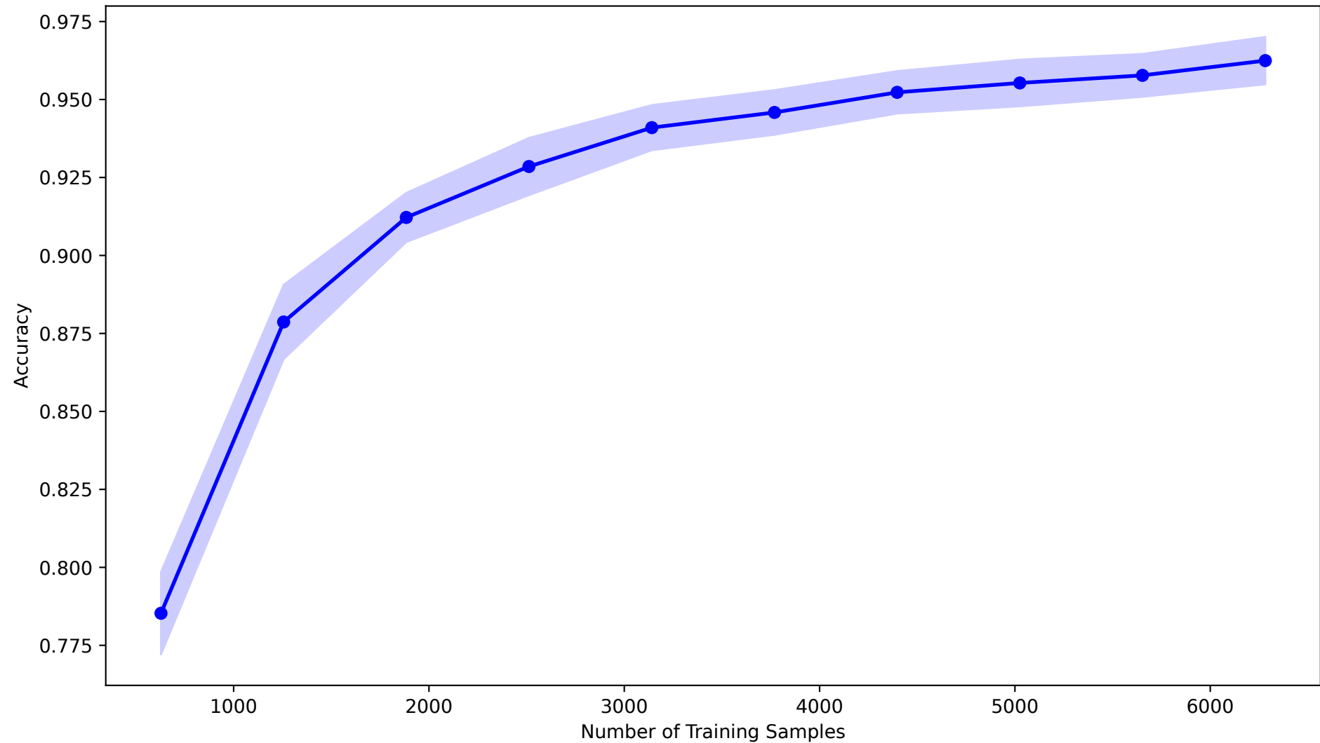
Random Forest Learning Curve - Material Accuracy
