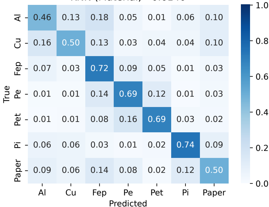
KNN (Material) - 0.6140
