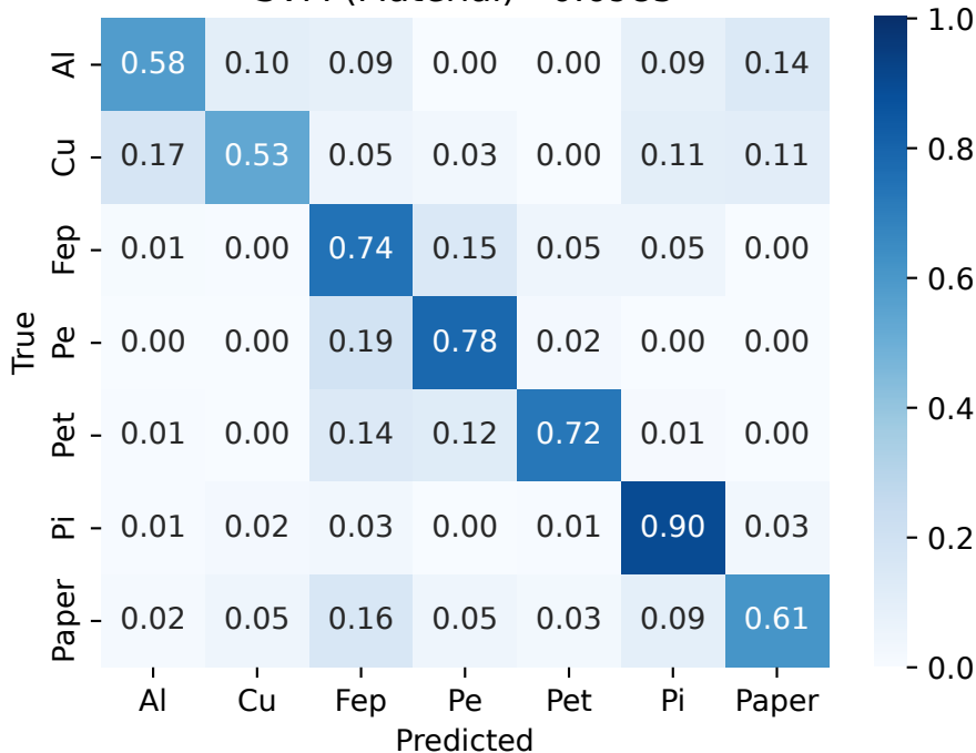
SVM (Material) - 0.6985
