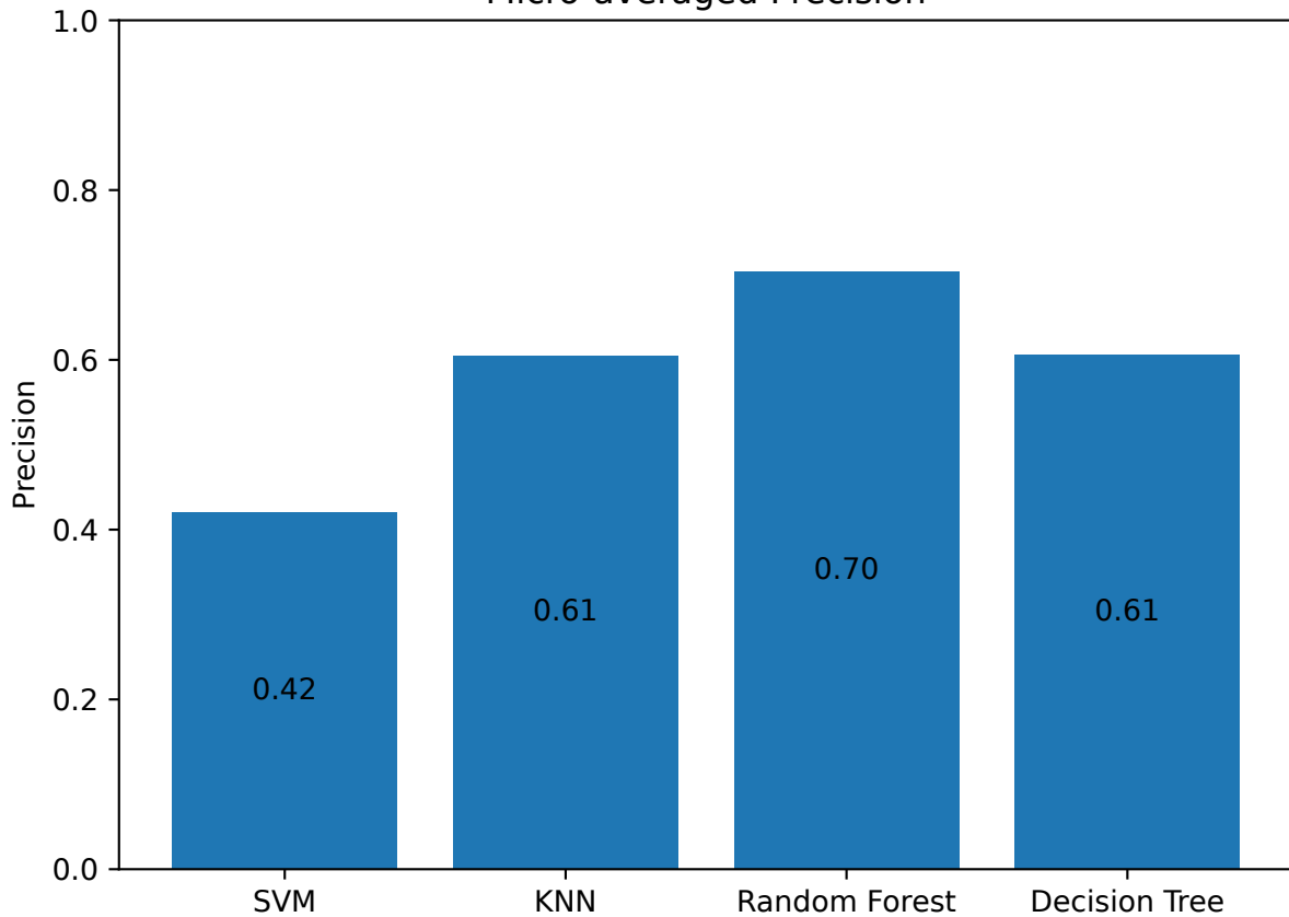
Micro-averaged Precision
