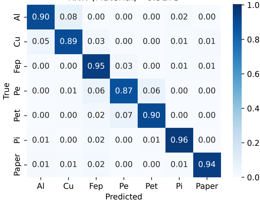
KNN (Material) - 0.9173
