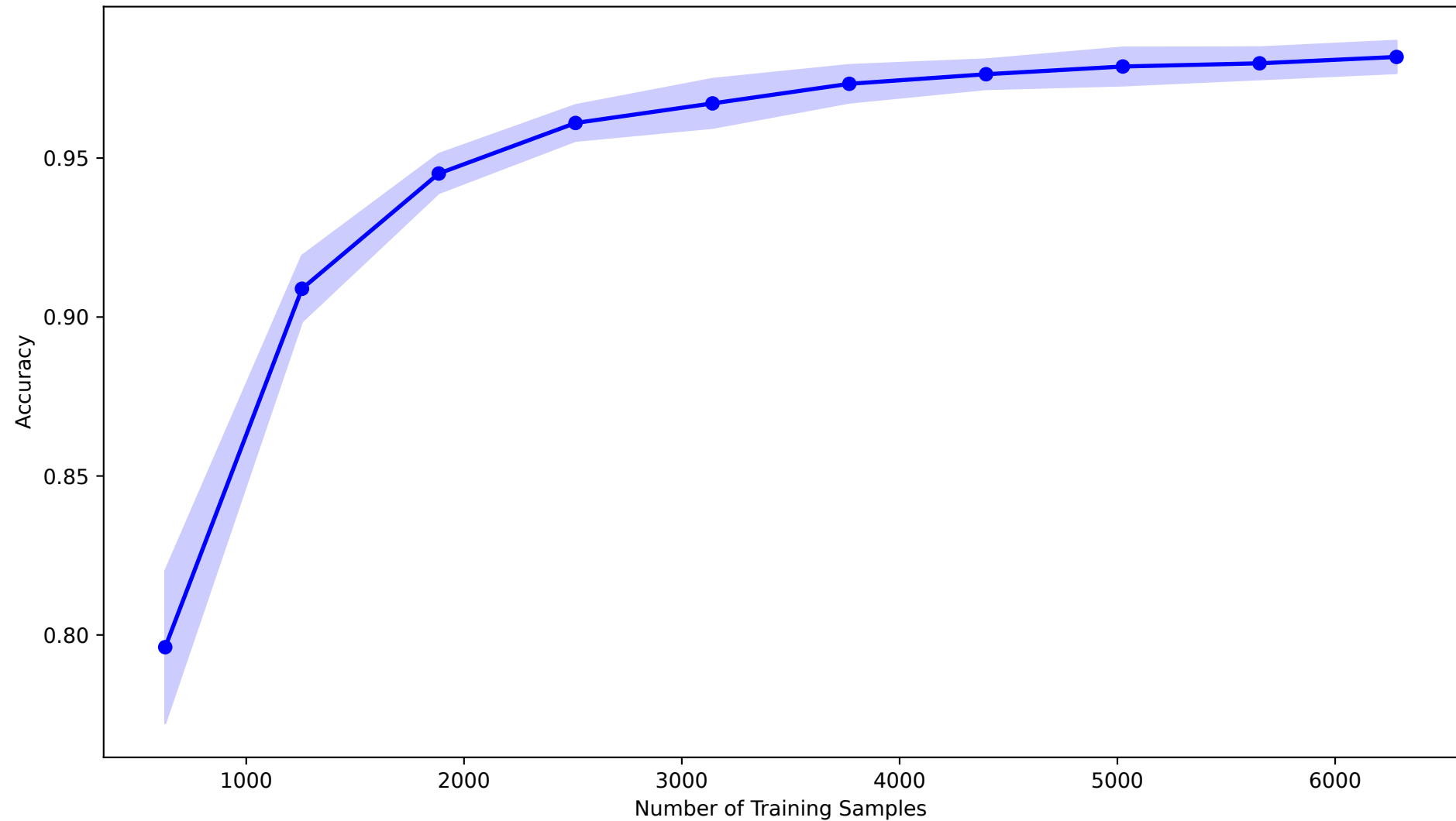
Random Forest Learning Curve - Overall Accuracy
