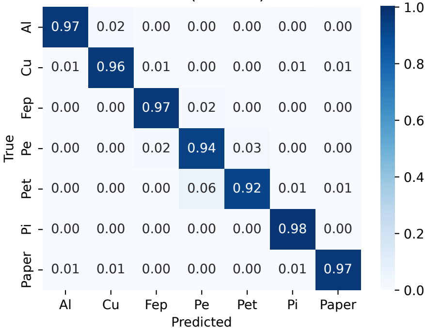
Random Forest (Material) - 0.9580
