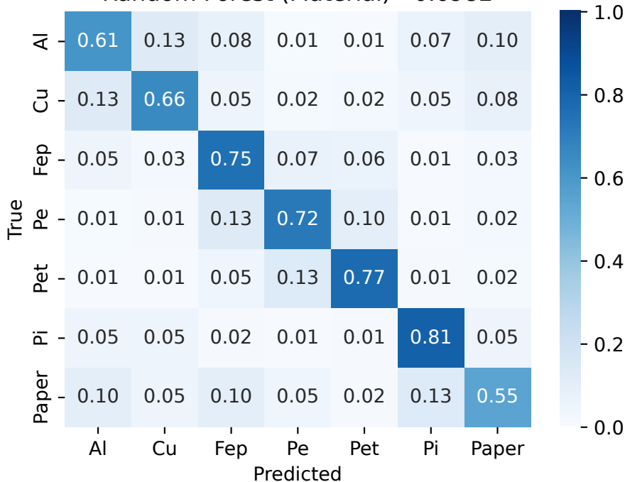
Random Forest (Material) - 0.6982
