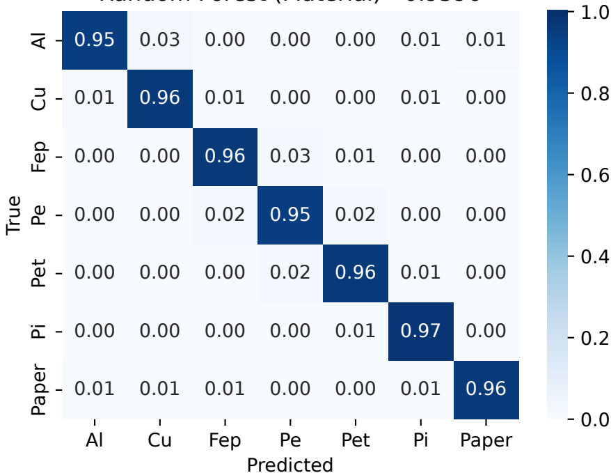
Random Forest (Material) - 0.9596
