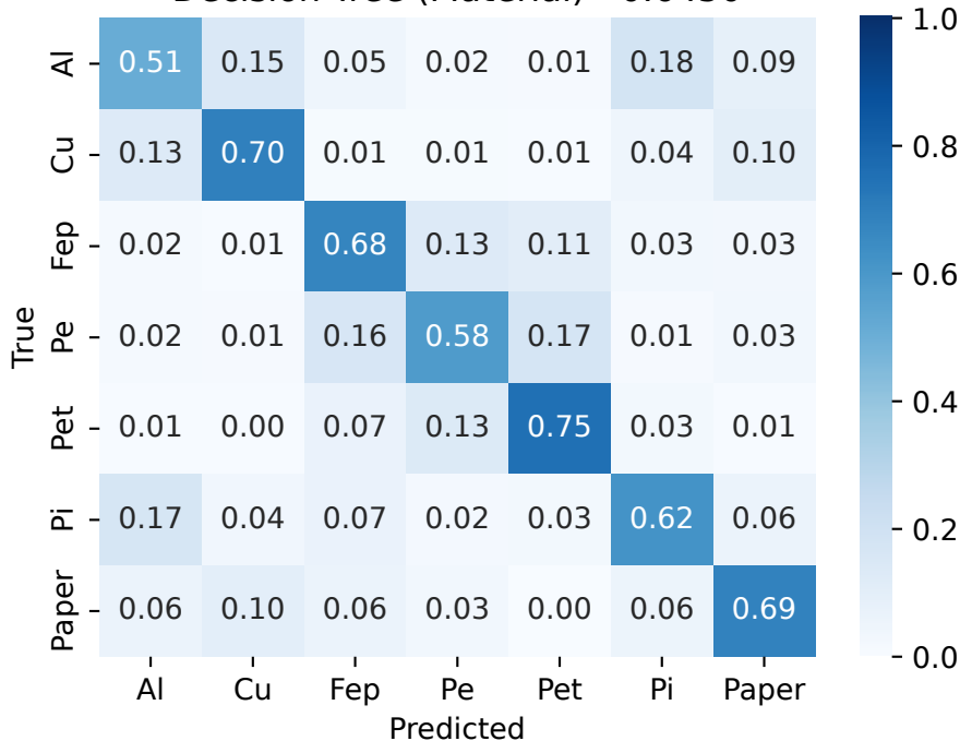
Decision Tree (Material) - 0.6450
