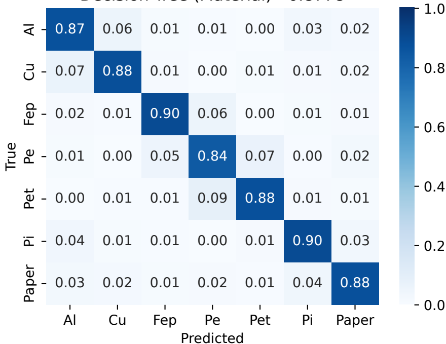
Decision Tree (Material) - 0.8778
