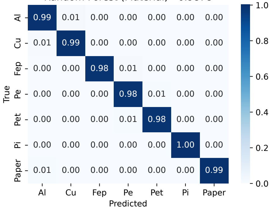
Random Forest (Material) - 0.9878
