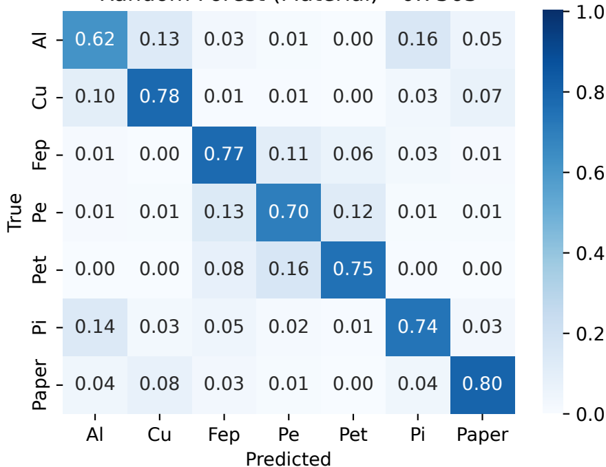
Random Forest (Material) - 0.7363
