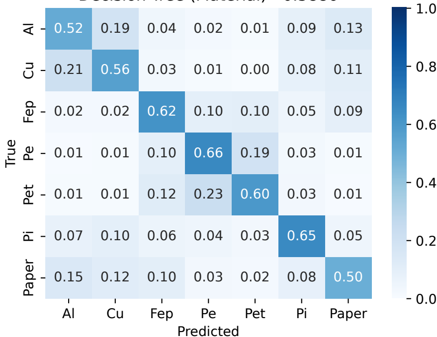
Decision Tree (Material) - 0.5886
