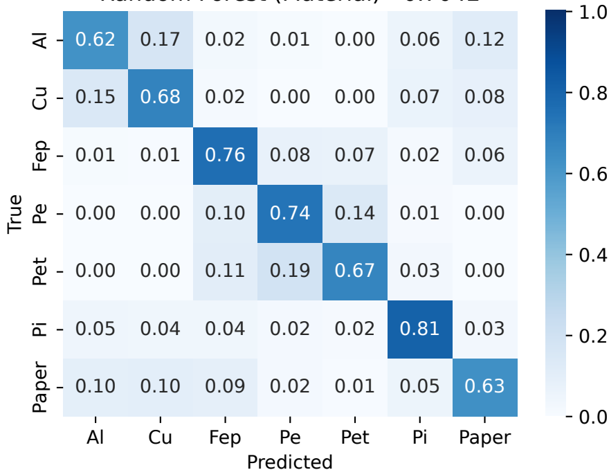
Random Forest (Material) - 0.7042
