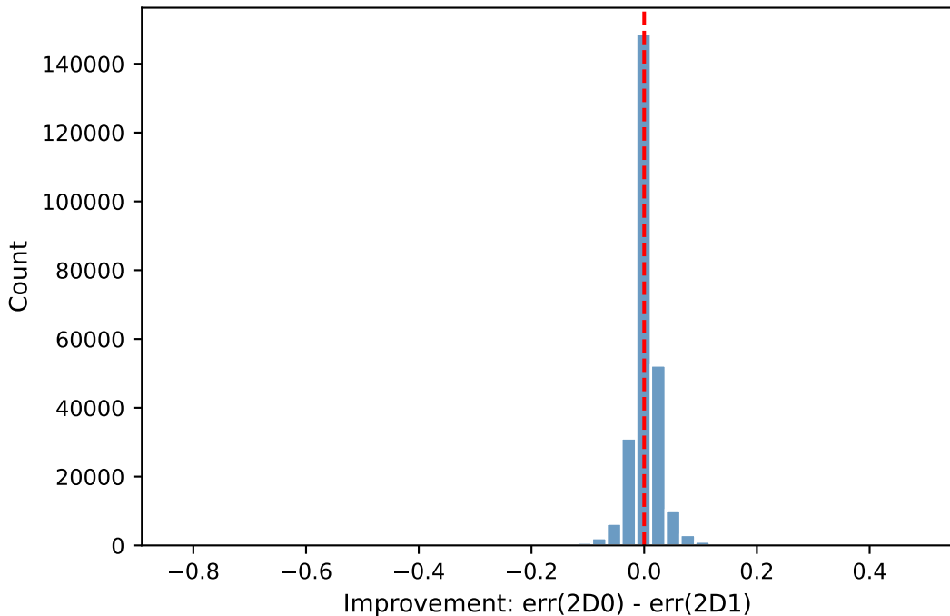
Distribution of Per-Sample Improvements
