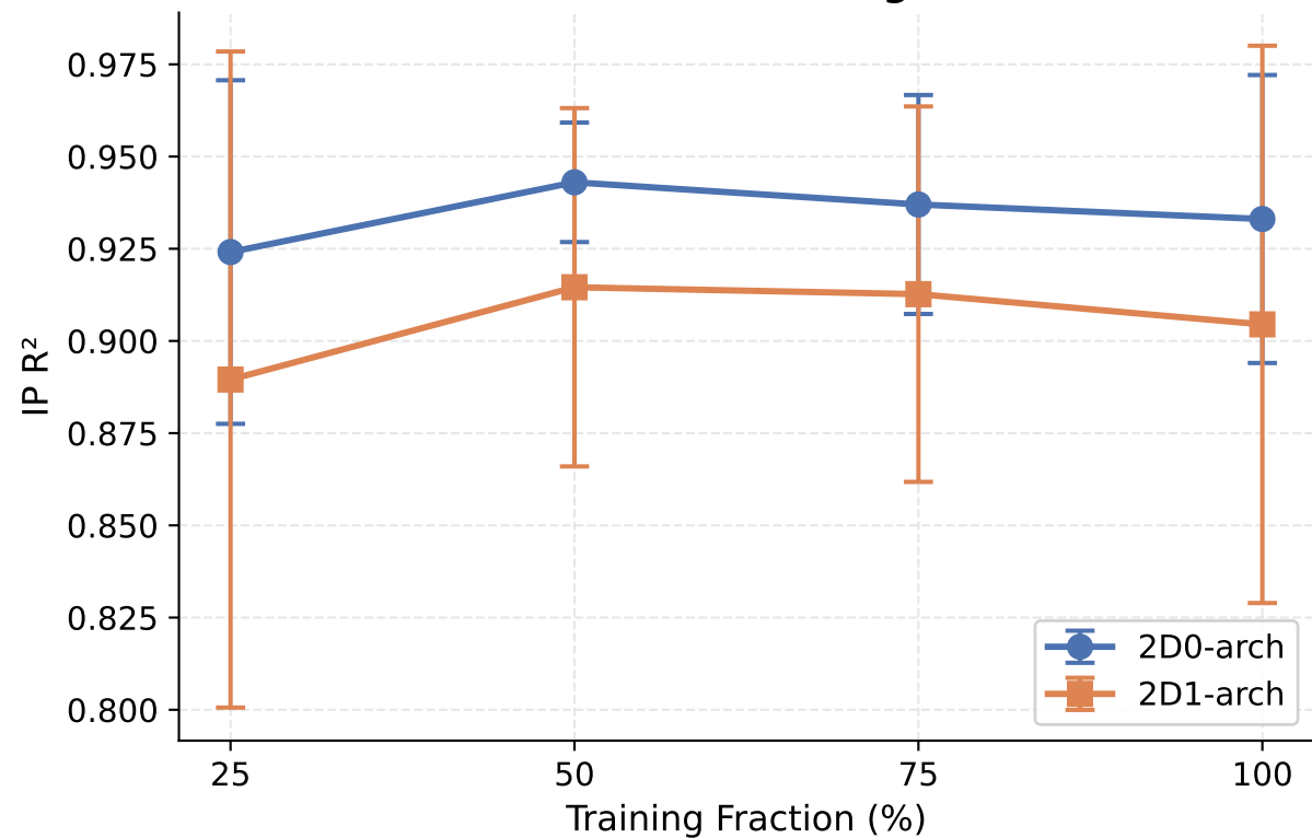
Overall IP R^2 vs Training Fraction
