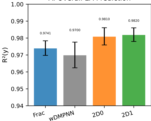
A. Overall EA Prediction
