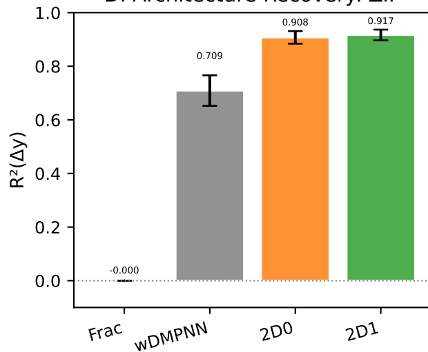
D. Architecture Recovery: \Delta IP
