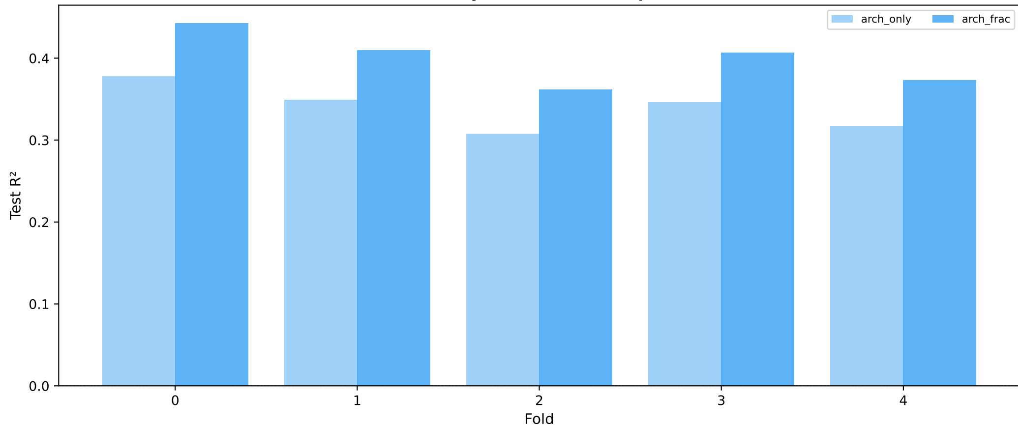
\Delta IP — Transfer R^2 by fold (best model per feature set)
