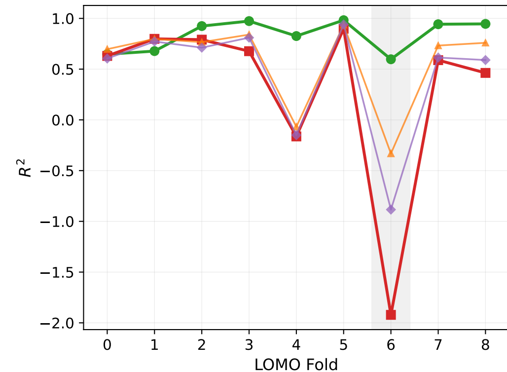
(c) EA Architecture-Deviation Prediction
