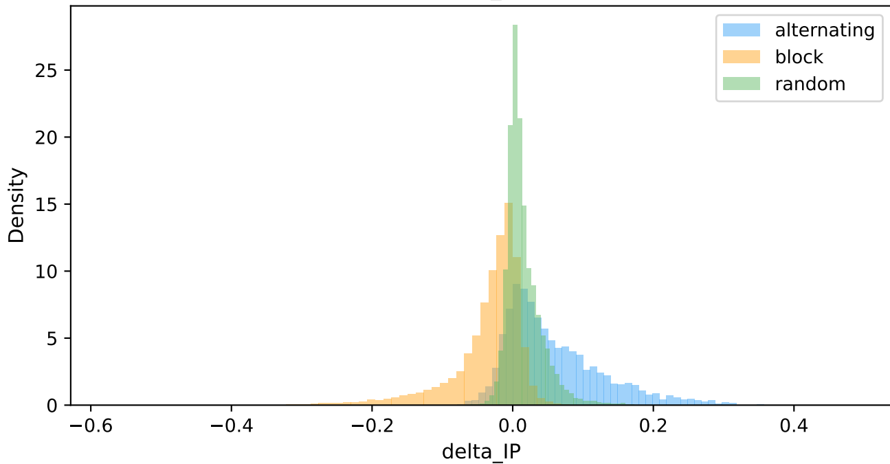
Distribution of delta_IP by architecture
