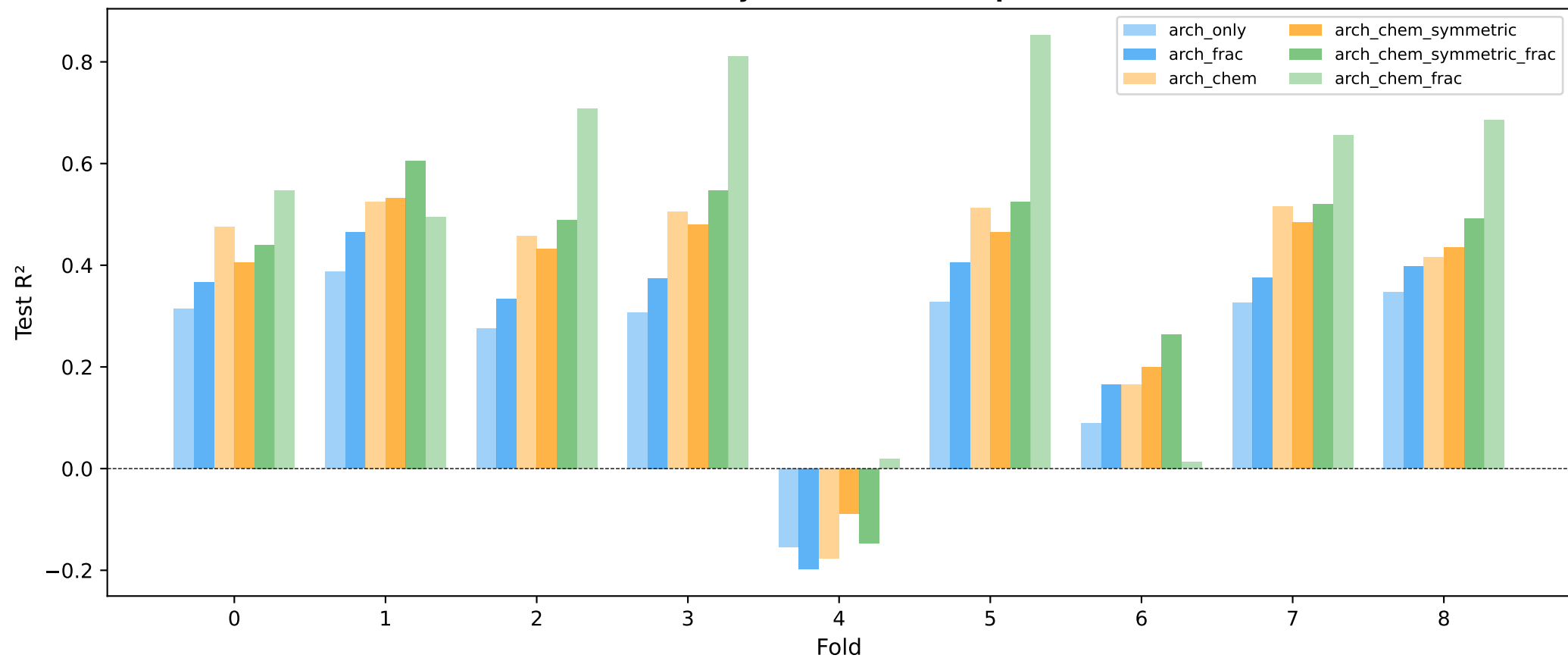
\Delta EA — Transfer R^2 by fold (best model per feature set)
