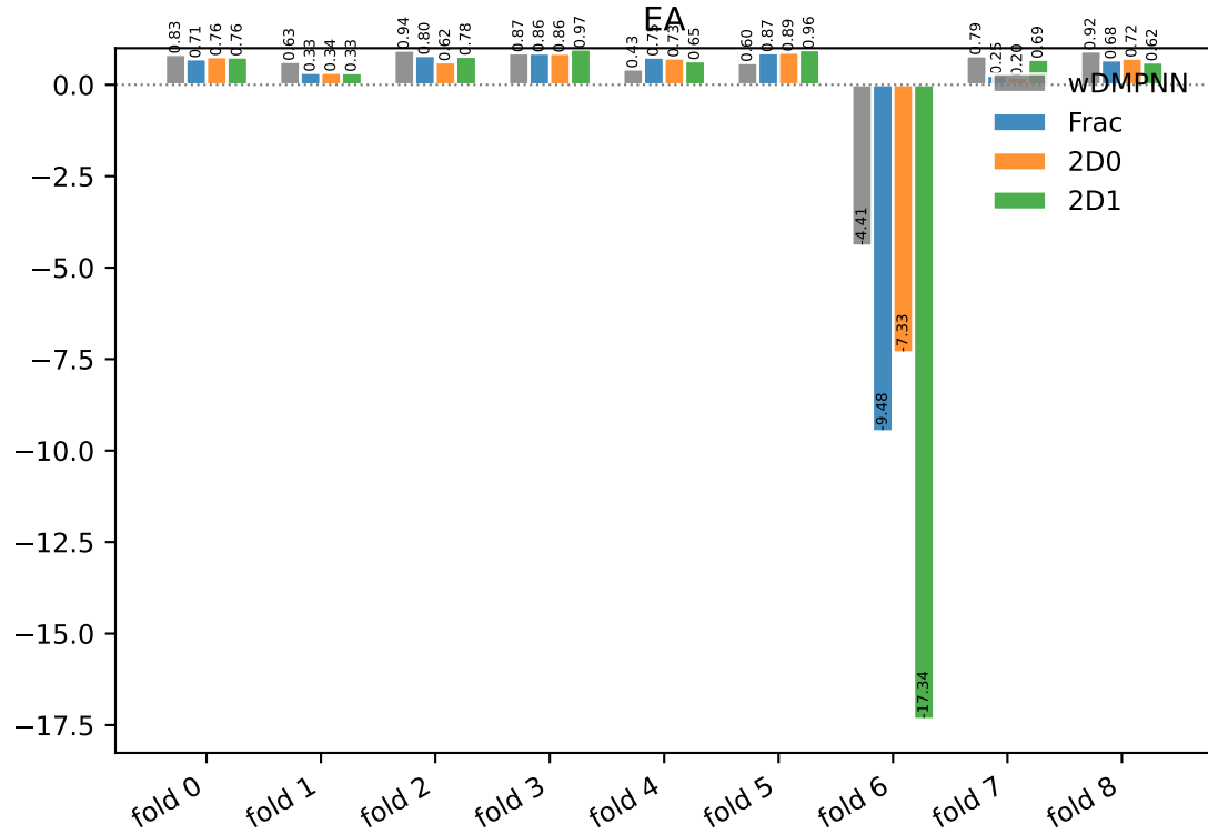
LOMO per-fold R^2
