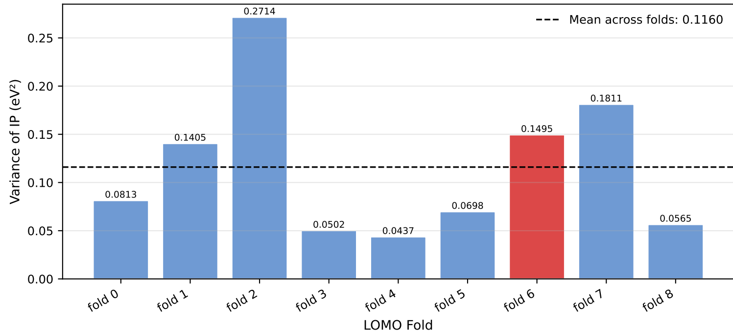
IP variance in test fold (split 6 = red)
