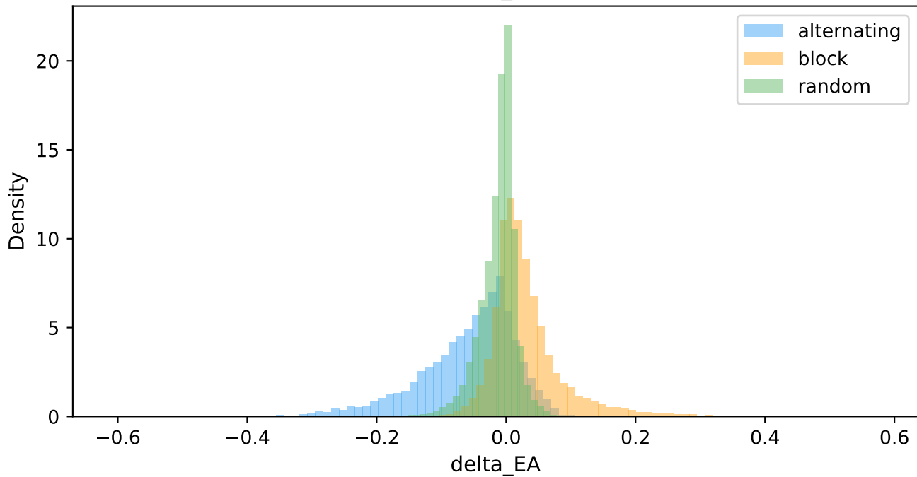
Distribution of delta_EA by architecture
