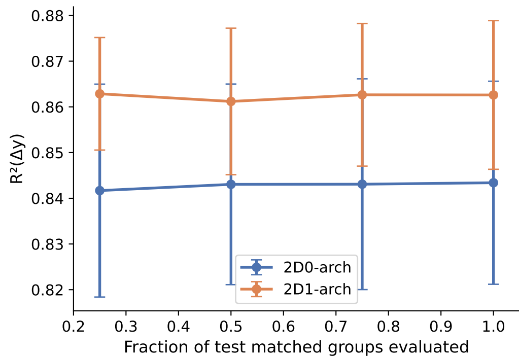
EA Architecture-Deviation R^2
