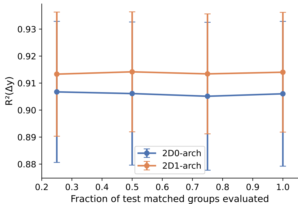
IP Architecture-Deviation R^2
