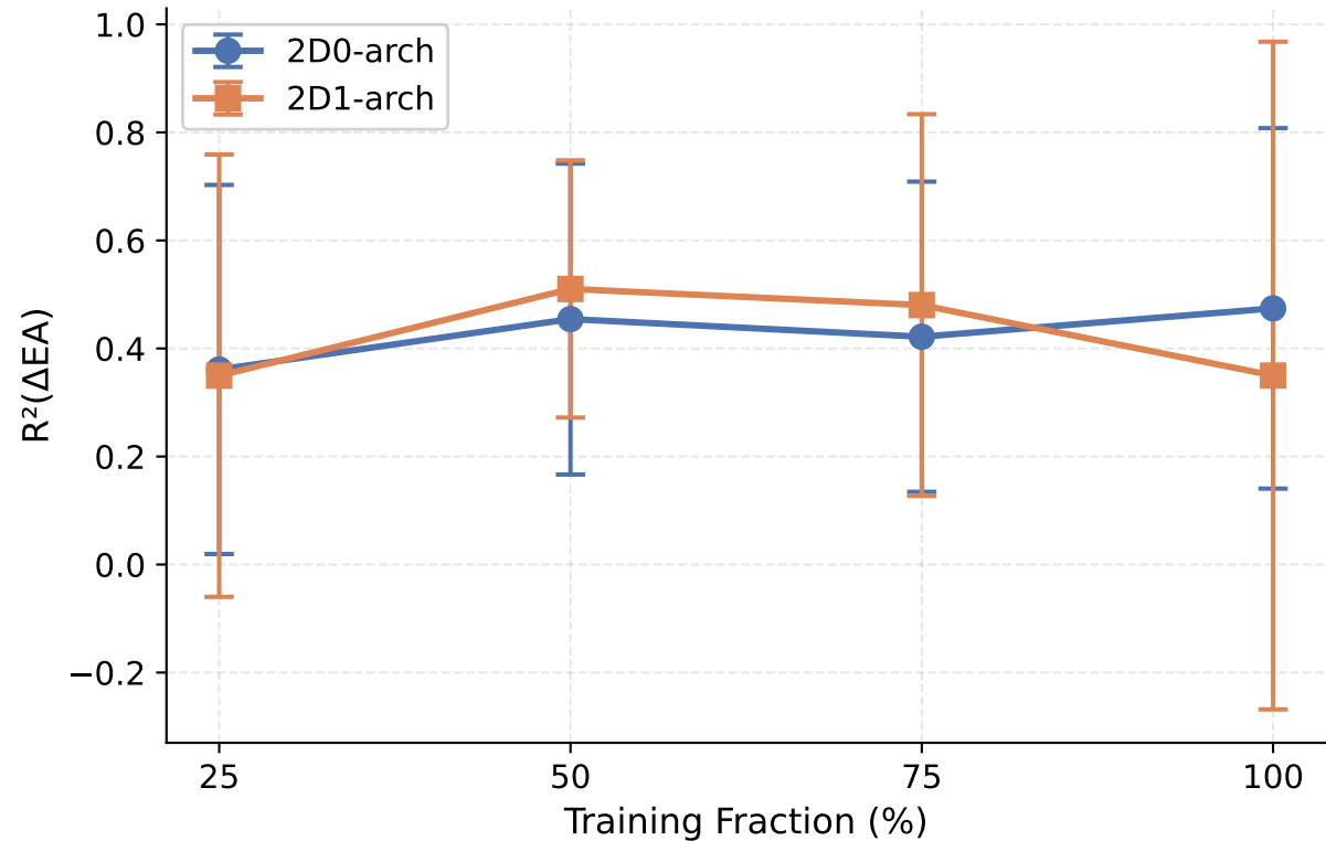
EA Architecture-Deviation R^2 vs Training Fraction
