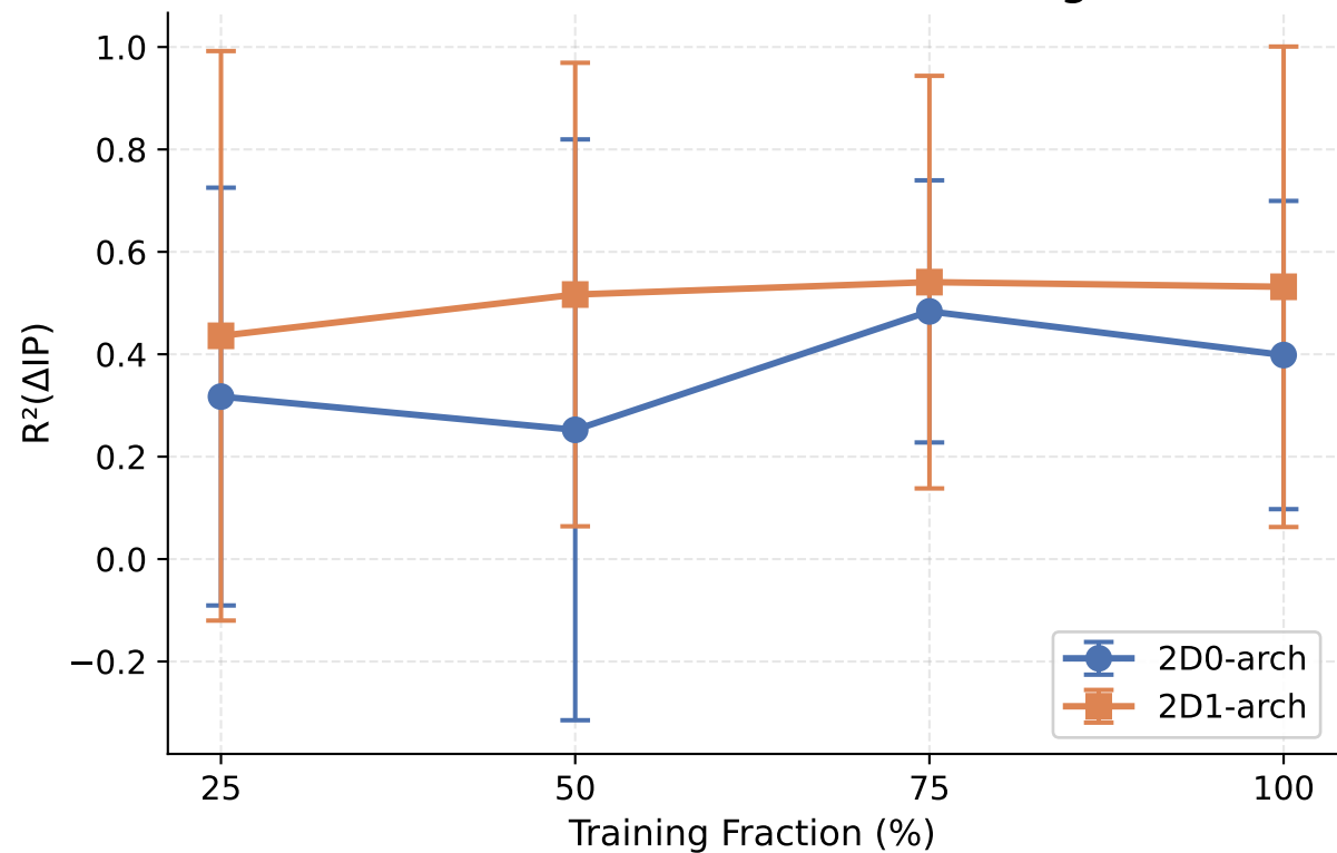
IP Architecture-Deviation R 2 vs Training Fraction
