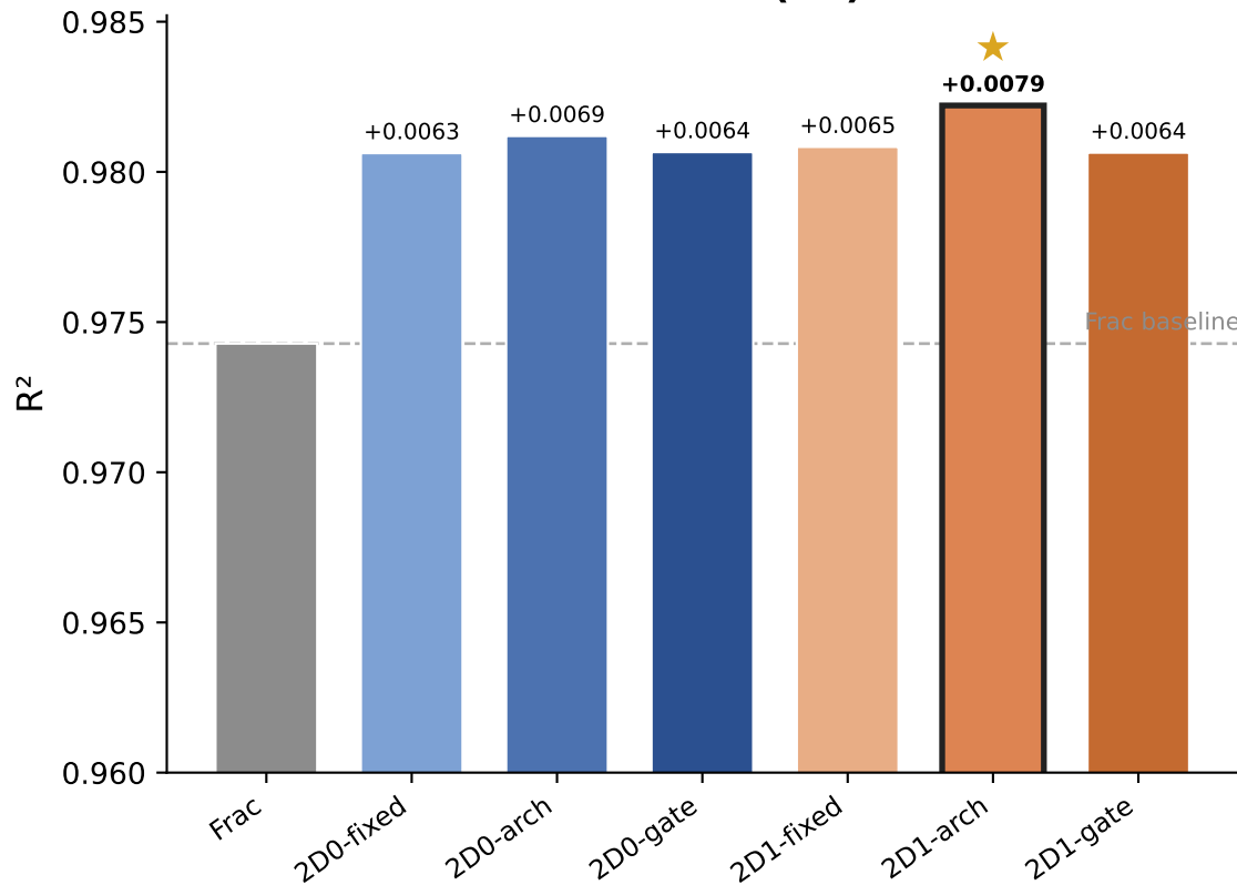
EA vs SHE (eV)
