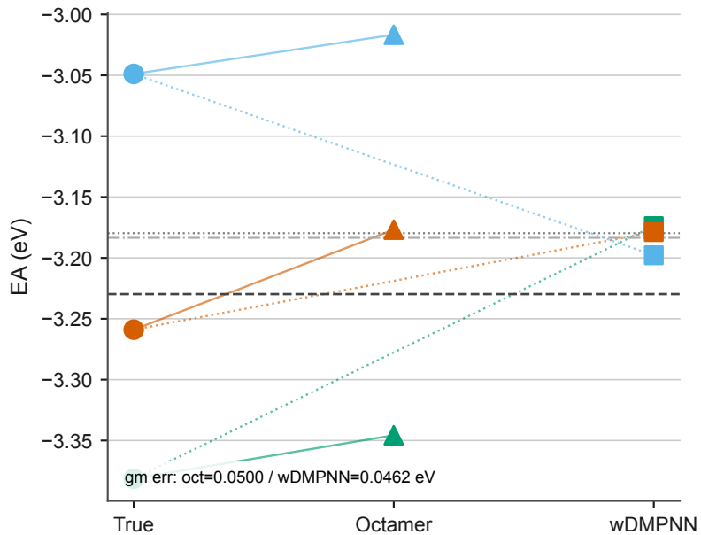
Chemistry placement
