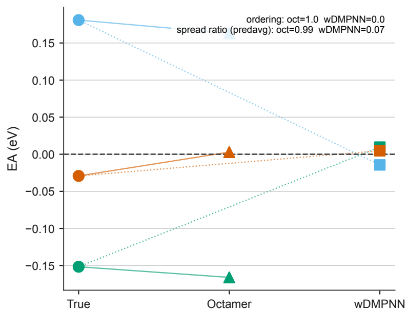
Architecture recovery
