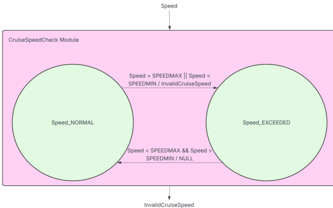
Fig. 4. CruiseSpeedCheck FSM
