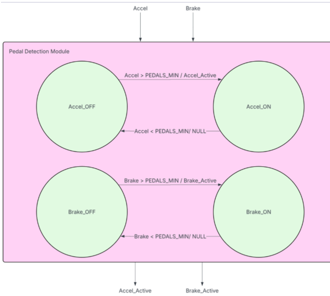
Fig. 3. Pedal Detection FSM
