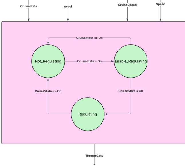
Fig. 6. car_driving_control FSM
