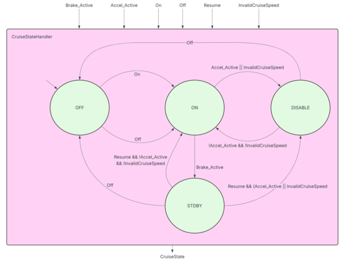
Fig. 5. CruiseStateHandler FSM
