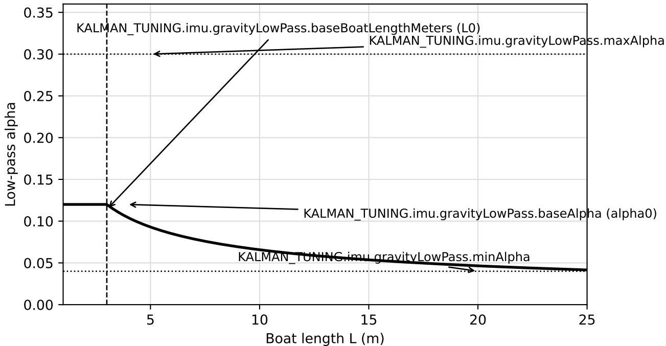
IMU gravity low-pass vs boat length
