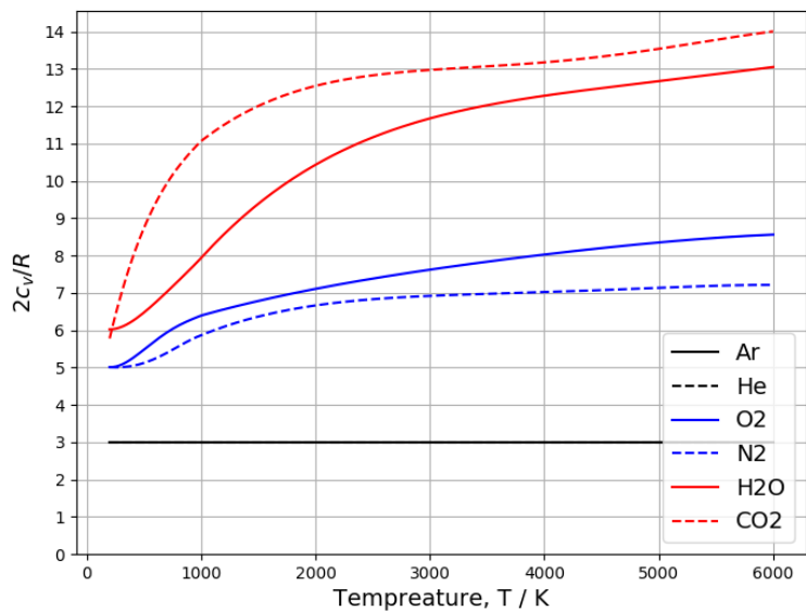
Figure 6.1: Approximate mean active degrees of freedom in selected ideal gas models
