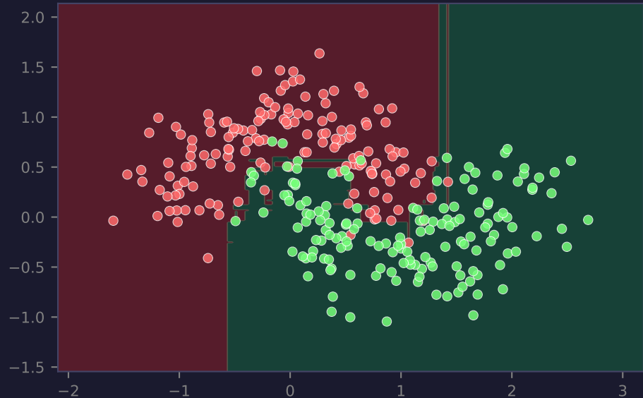
Gradient Boosting
